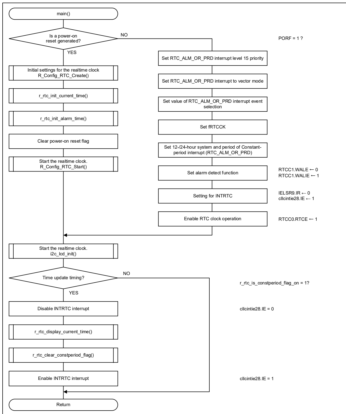
Figure 4.1 main Processing
