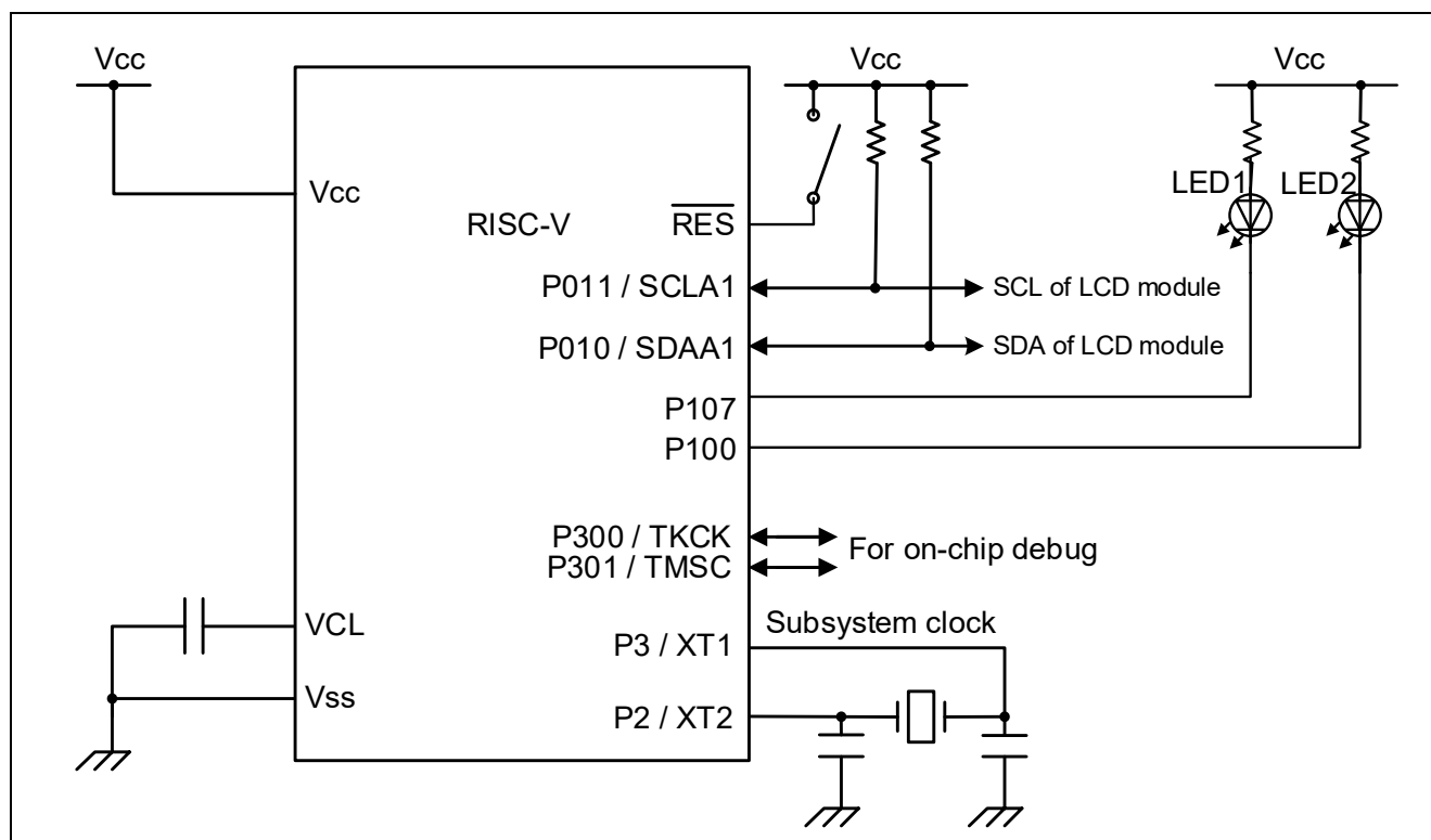
Figure 3.1 Hardware Configuration
