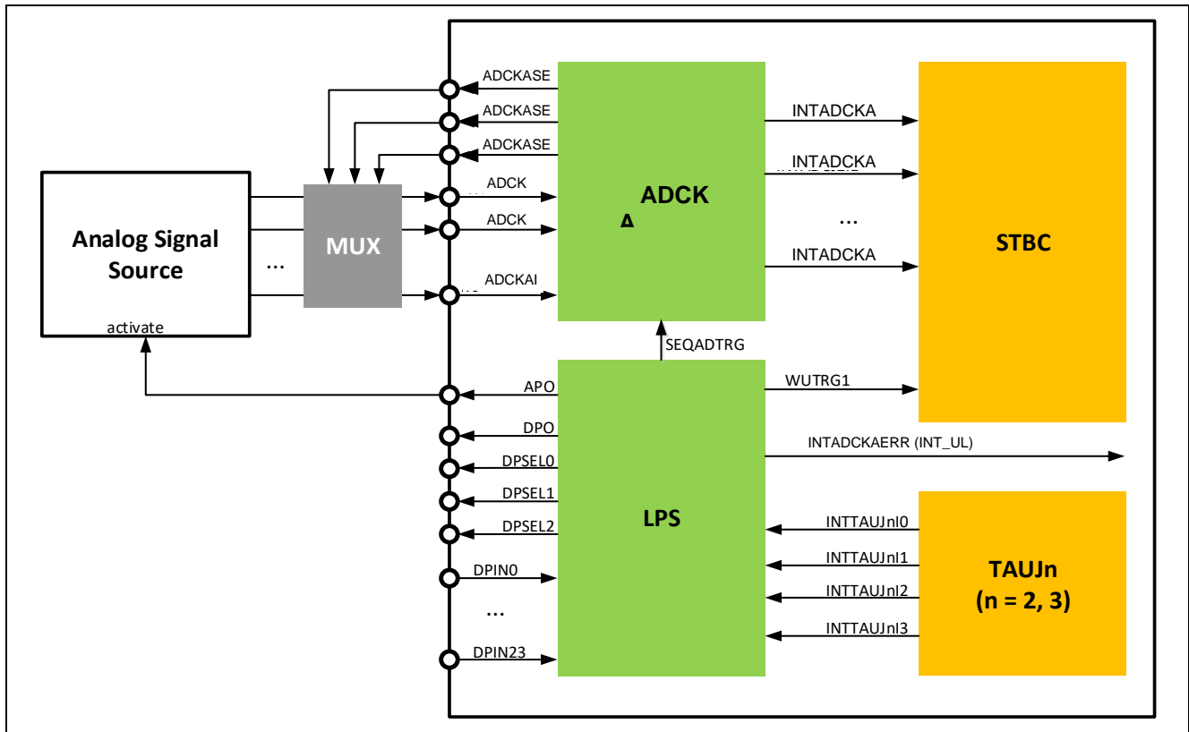
Figure 6-3 Block Diagram for the Analog Input Mode of LPS
