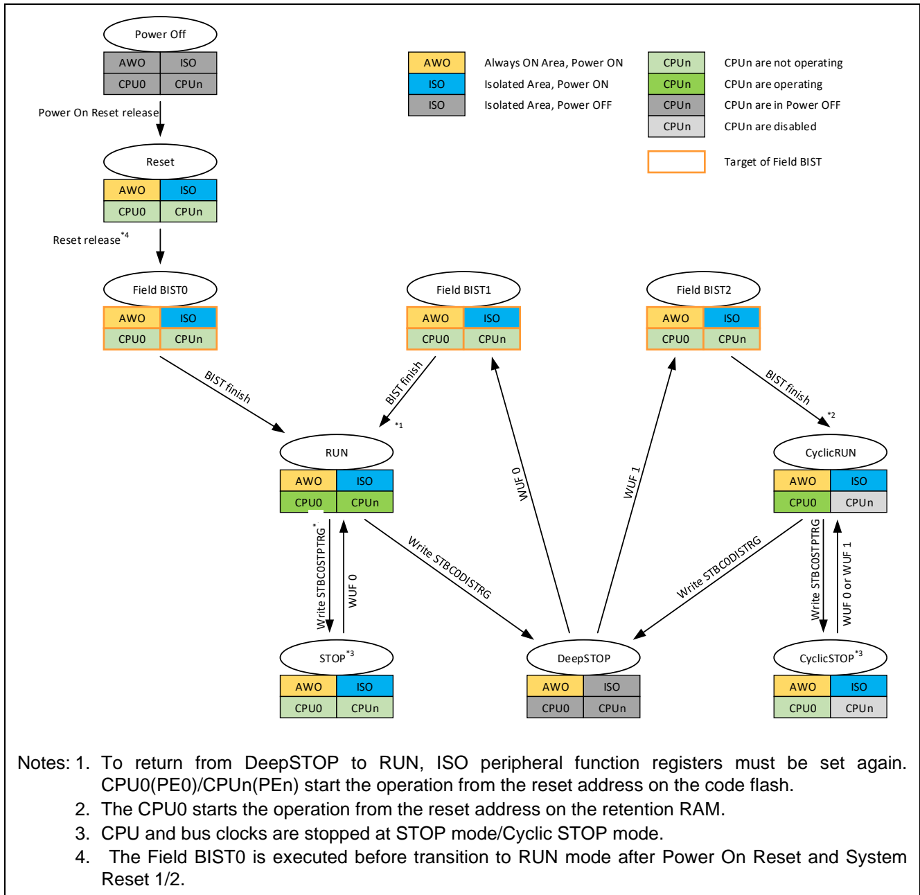
Figure 4-1 Transition to Chip Standby Modes
