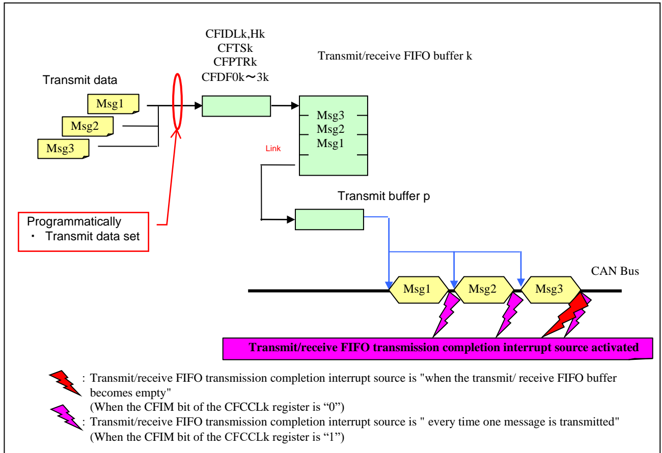
Figure 3-1 Operation of Transmit/receive FIFO Buffer (Transmit mode)
