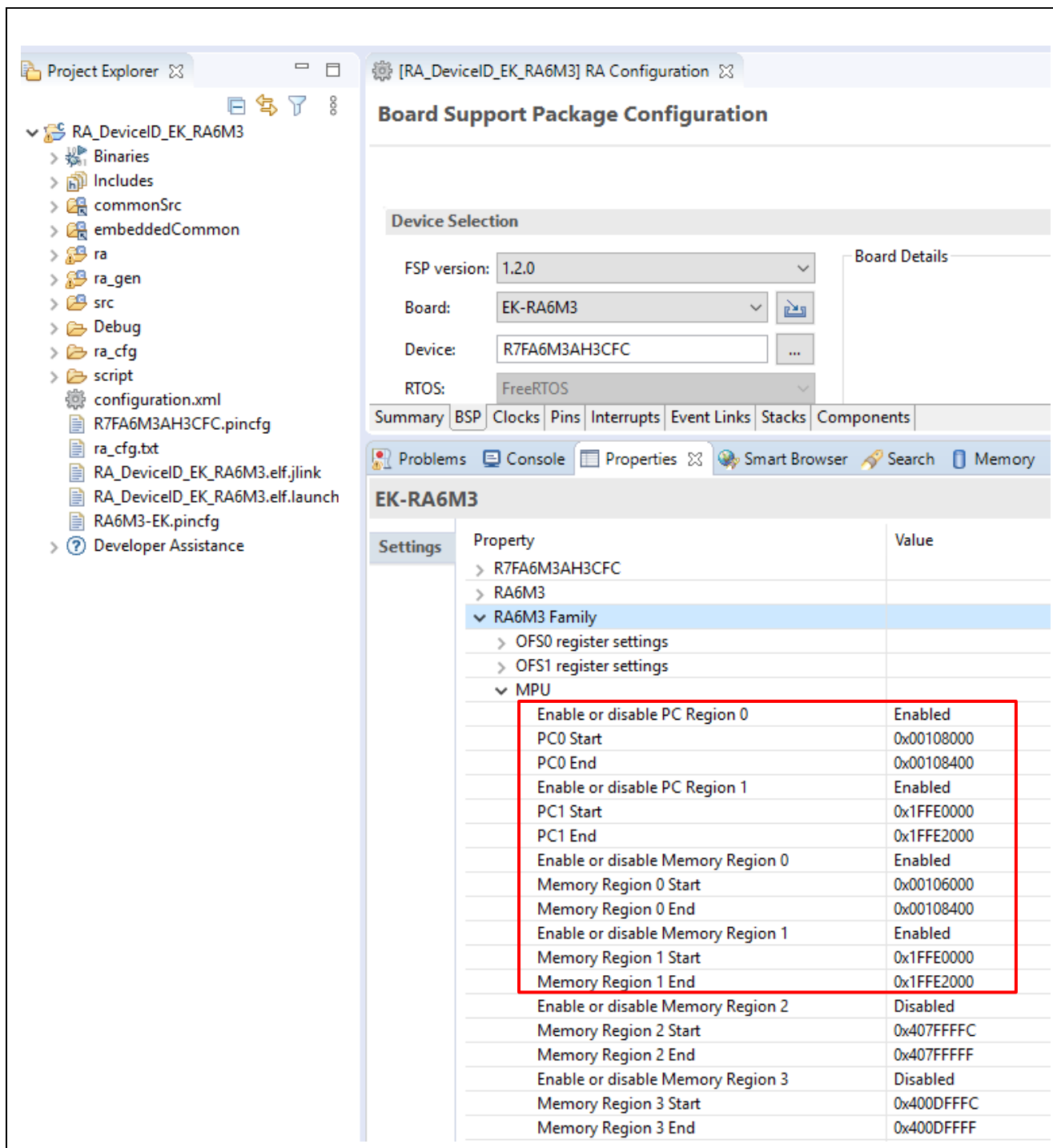
Figure 6. Security MPU settings using e 2 studio ISDE Configurator
