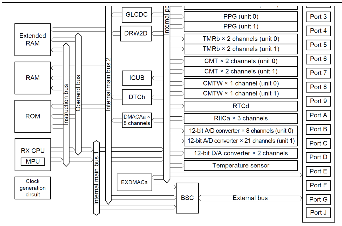
Figure 2.2 RX65N System Block Diagram (Detail View)
