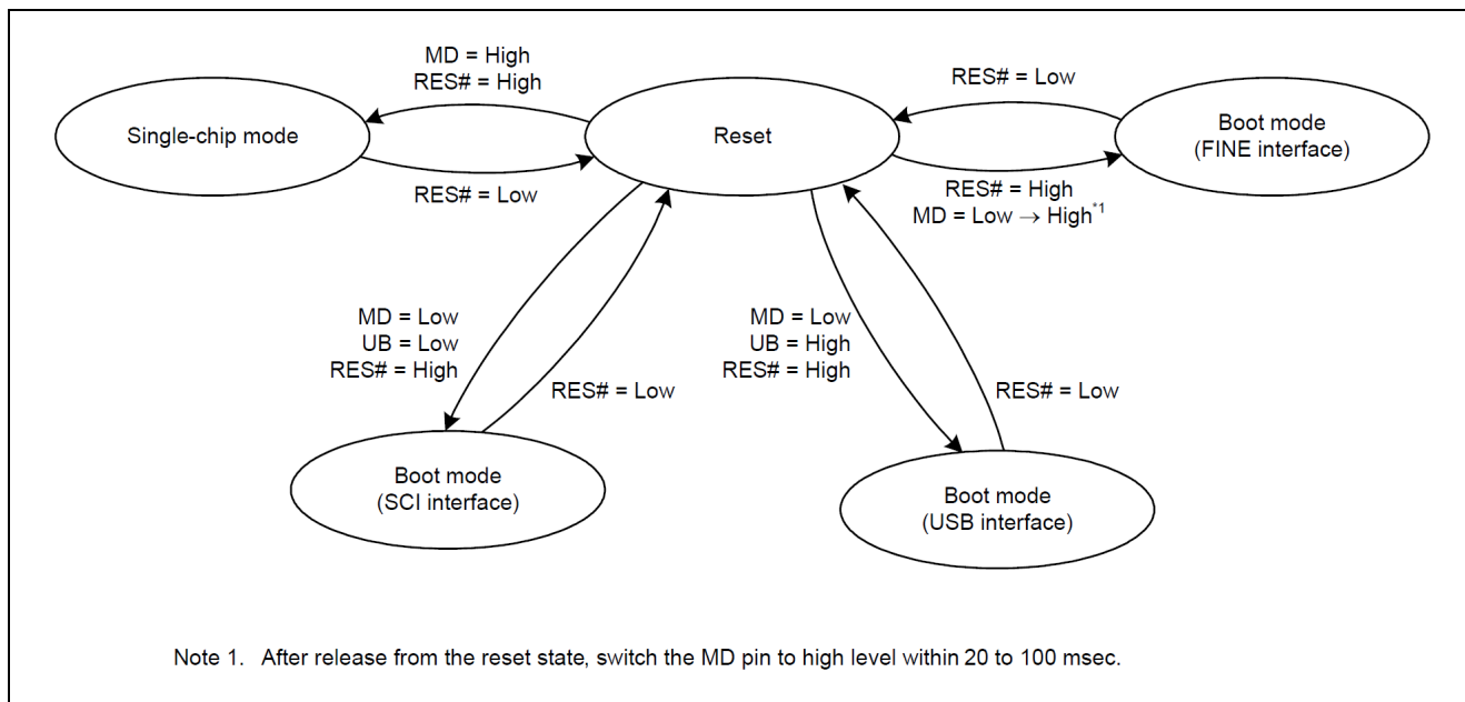
Figure 3.2 Excerpt of RX65N Flash Memory Specifications
