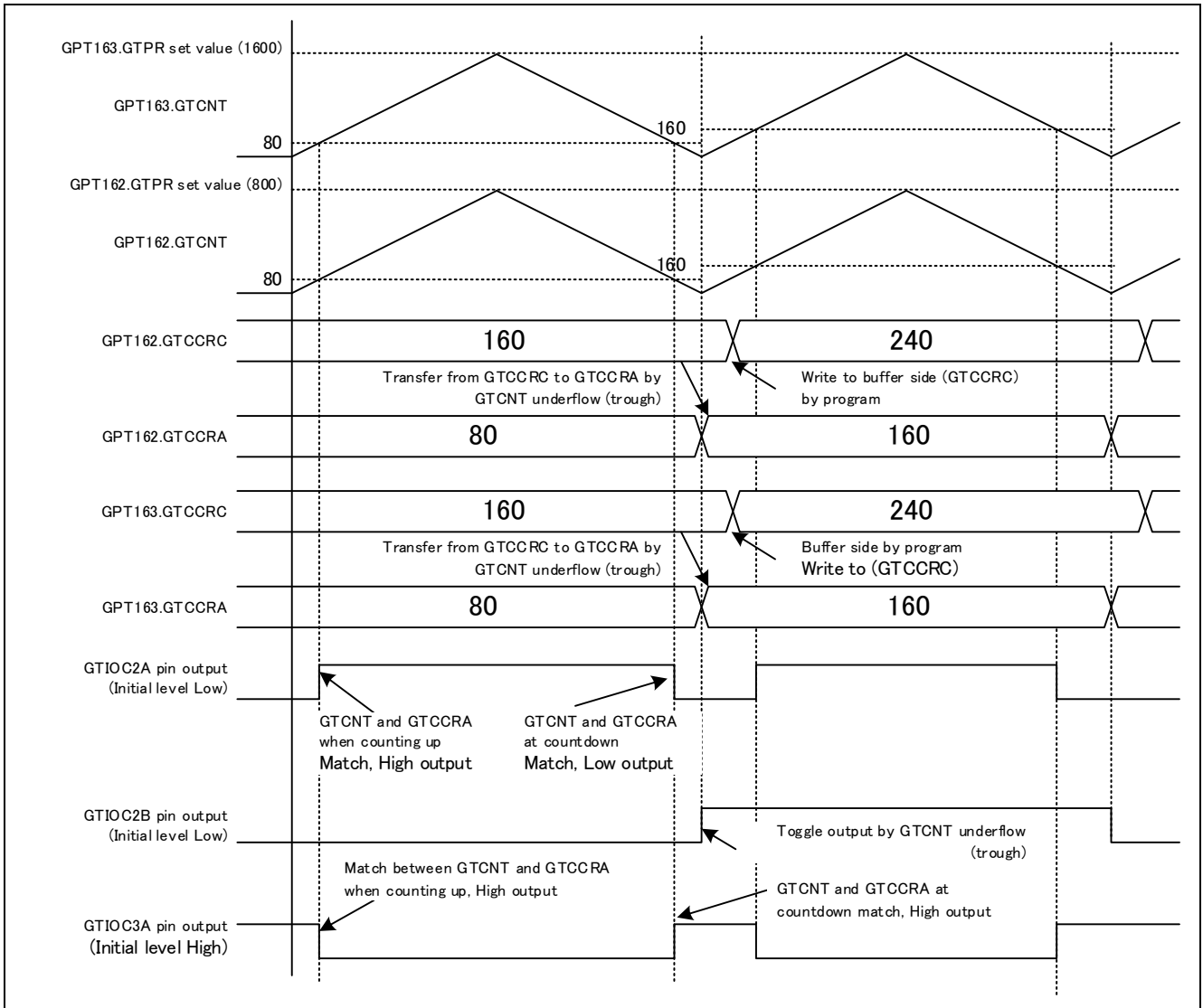
Figure 1.1 GPT output waveform
