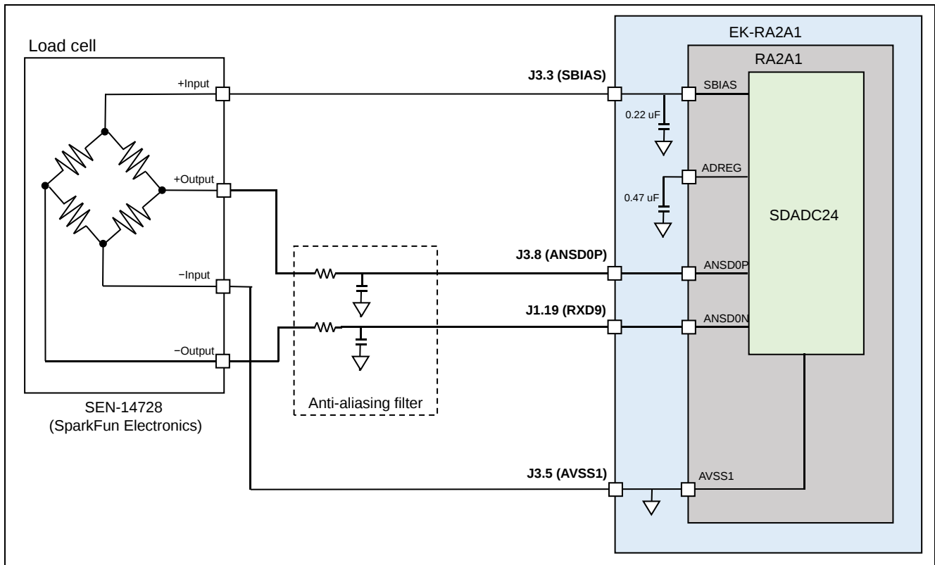
Figure 4-1 Example of Connections with the EK-RA2A1 Board
