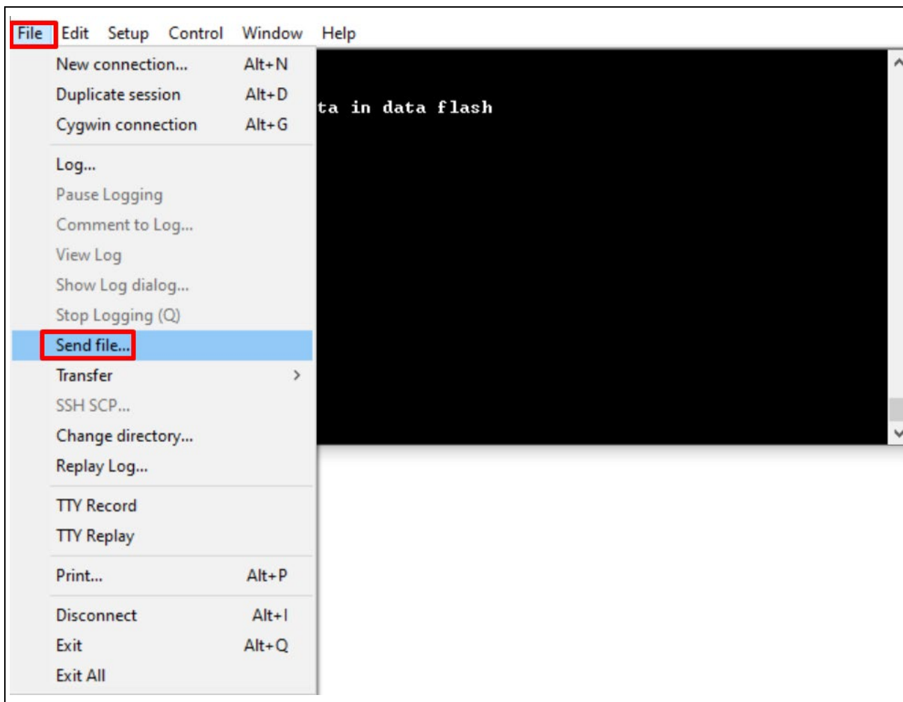
Figure 51. Send File Option in File Menu
