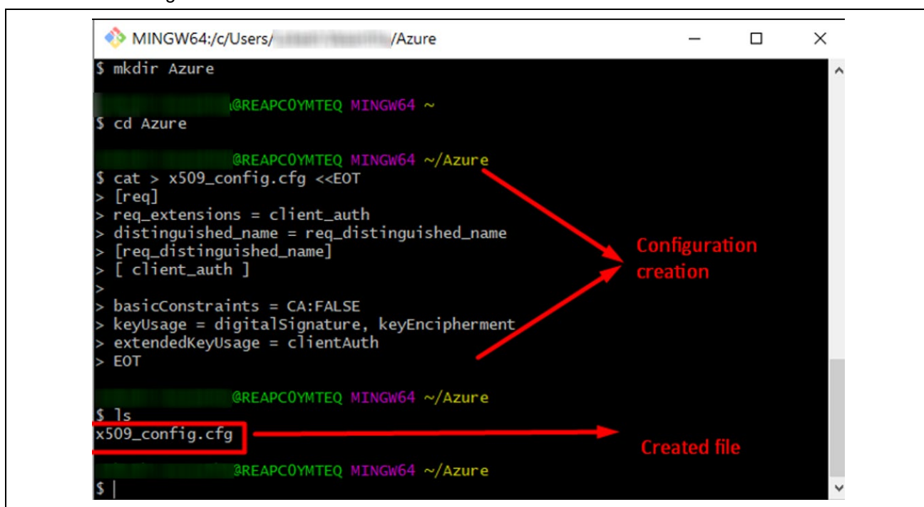
Figure 16. Set X509 Configuration File
