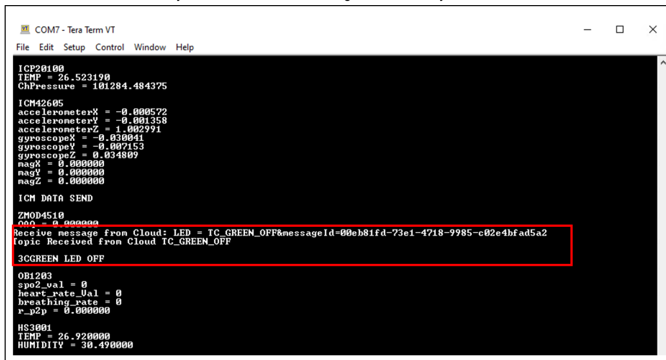
Figure 61. Serial Terminal Output
