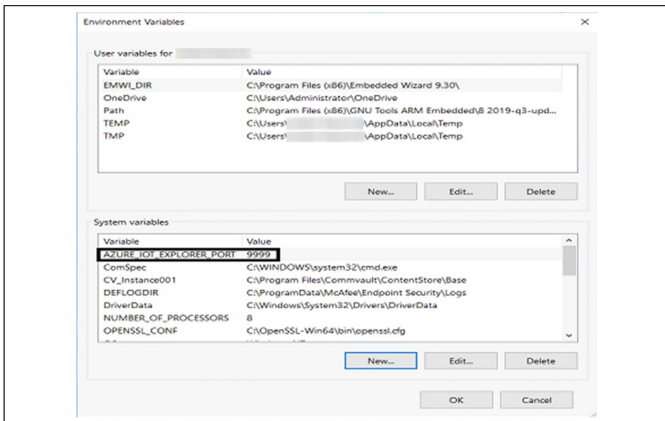
Figure 28. Added Alternate Port for Azure IoT Explorer
