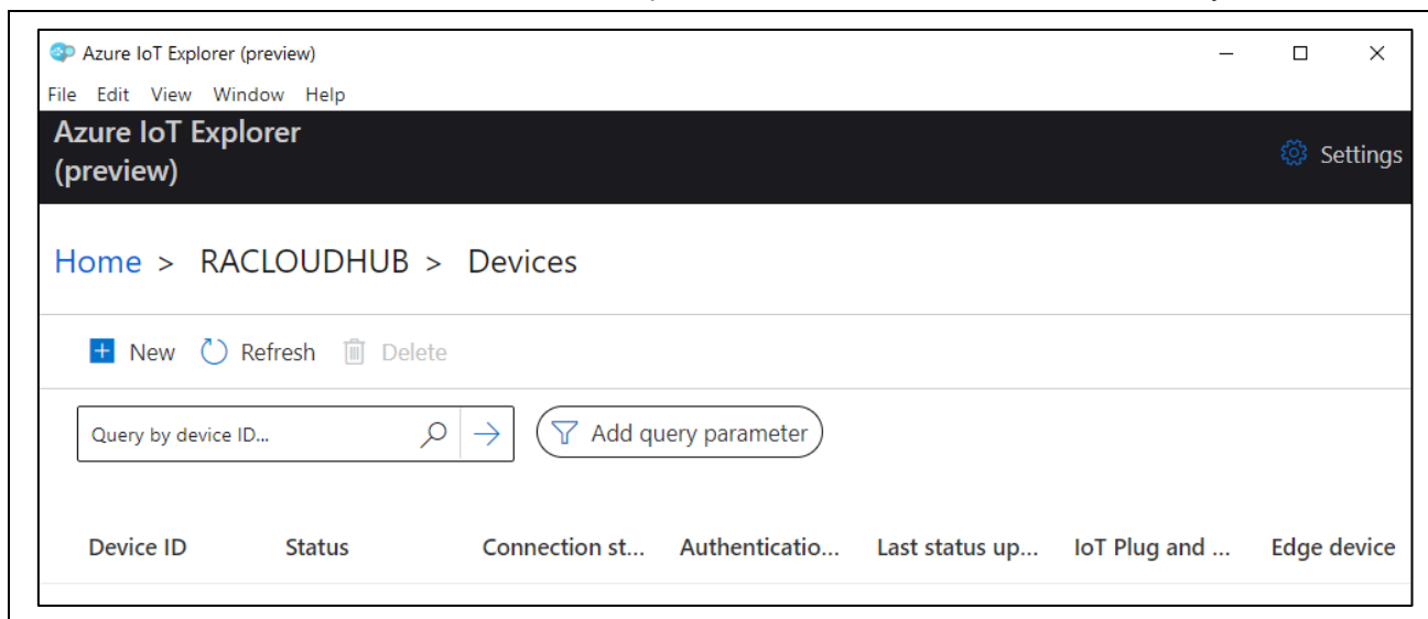
Figure 29. Listed Devices
