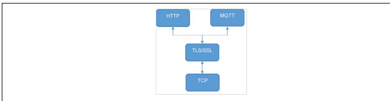
Figure 5. SSL/TLS Hierarchy
