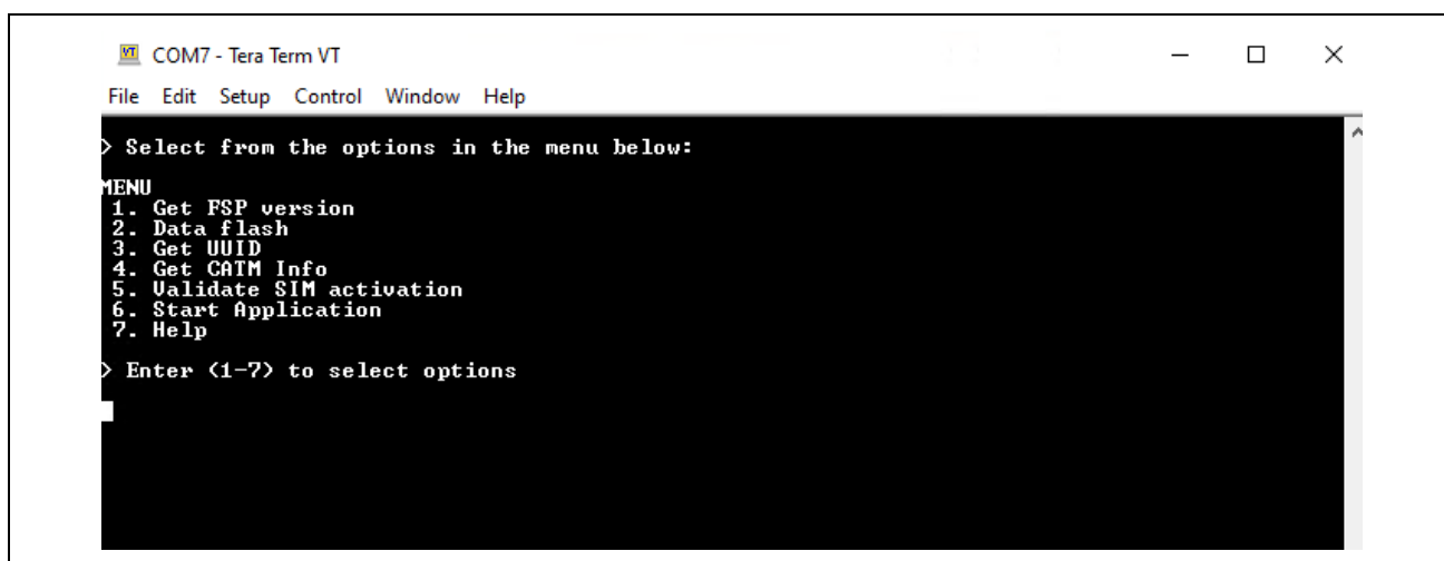
Figure 42. Main Menu
