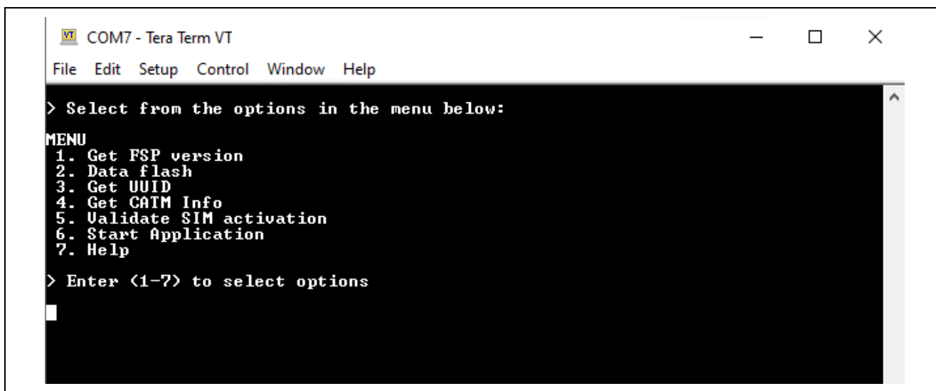
Figure 48. Main Menu
