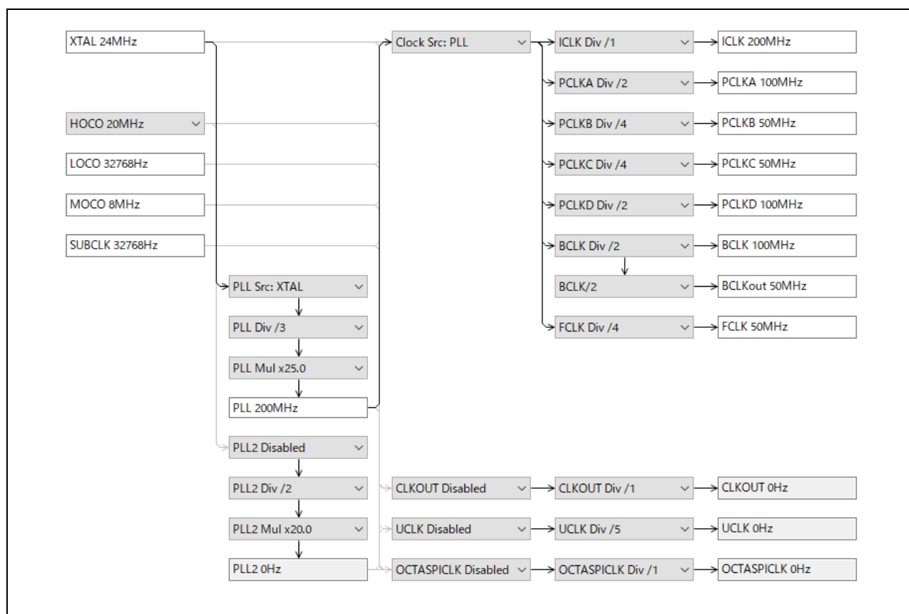
Figure 3.1 Clock Configuration
