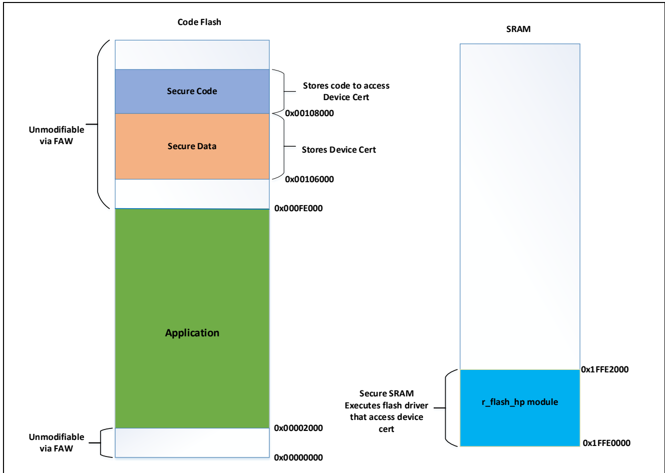
Figure 5. Memory Map used in the Application Project
