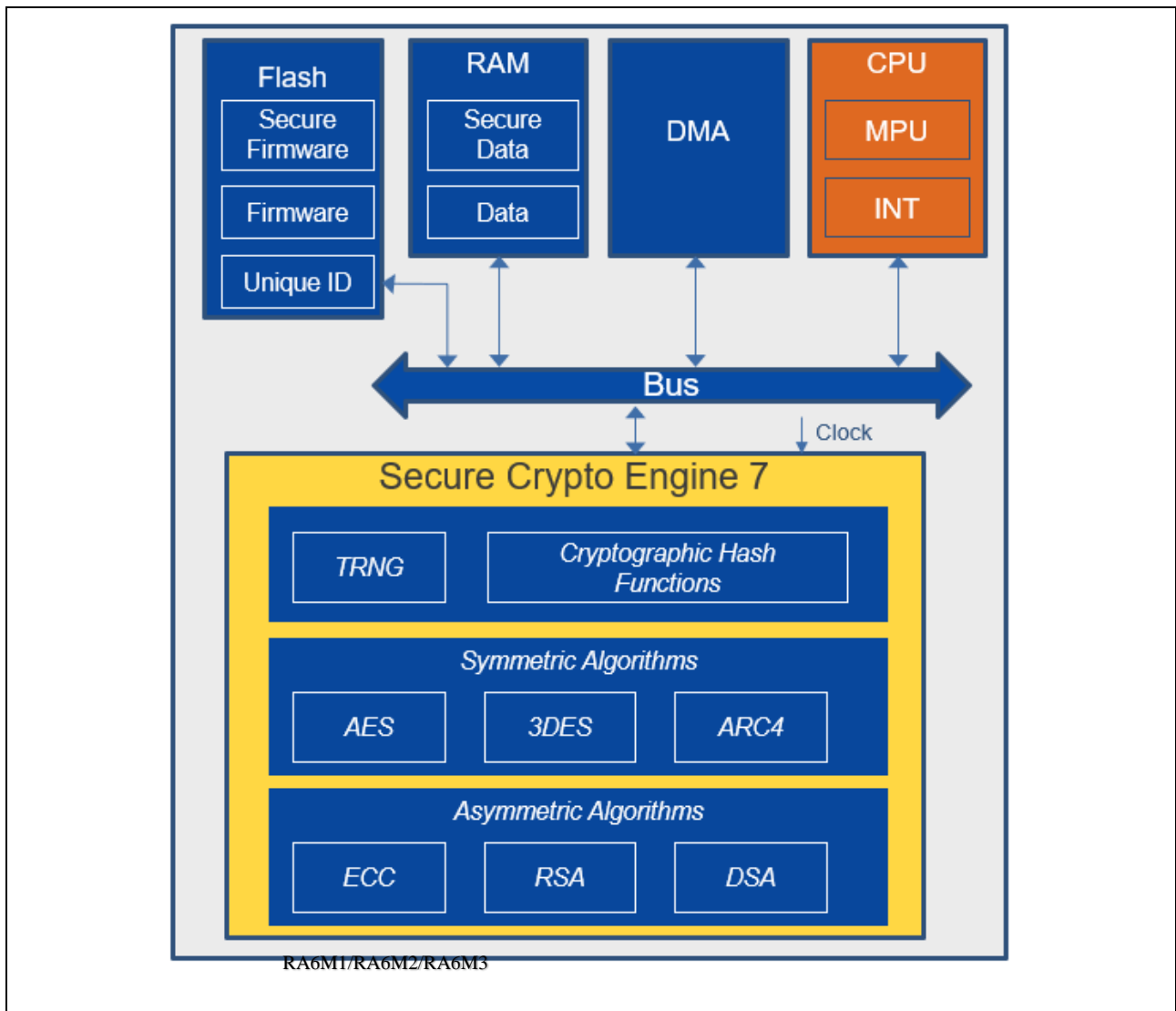
Figure 2. Security Hardware Peripherals Available in RA6M1/2/3
