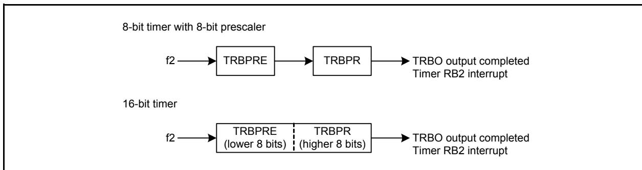
Figure 3.1 Block Diagram
