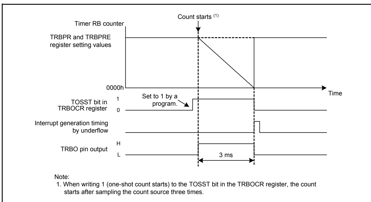
Figure 3.2 Timing Diagram
