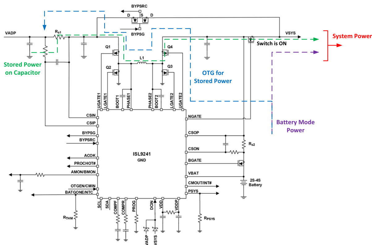
Figure 5. Supplemental Mode (Intel VMIN Active Protection)
