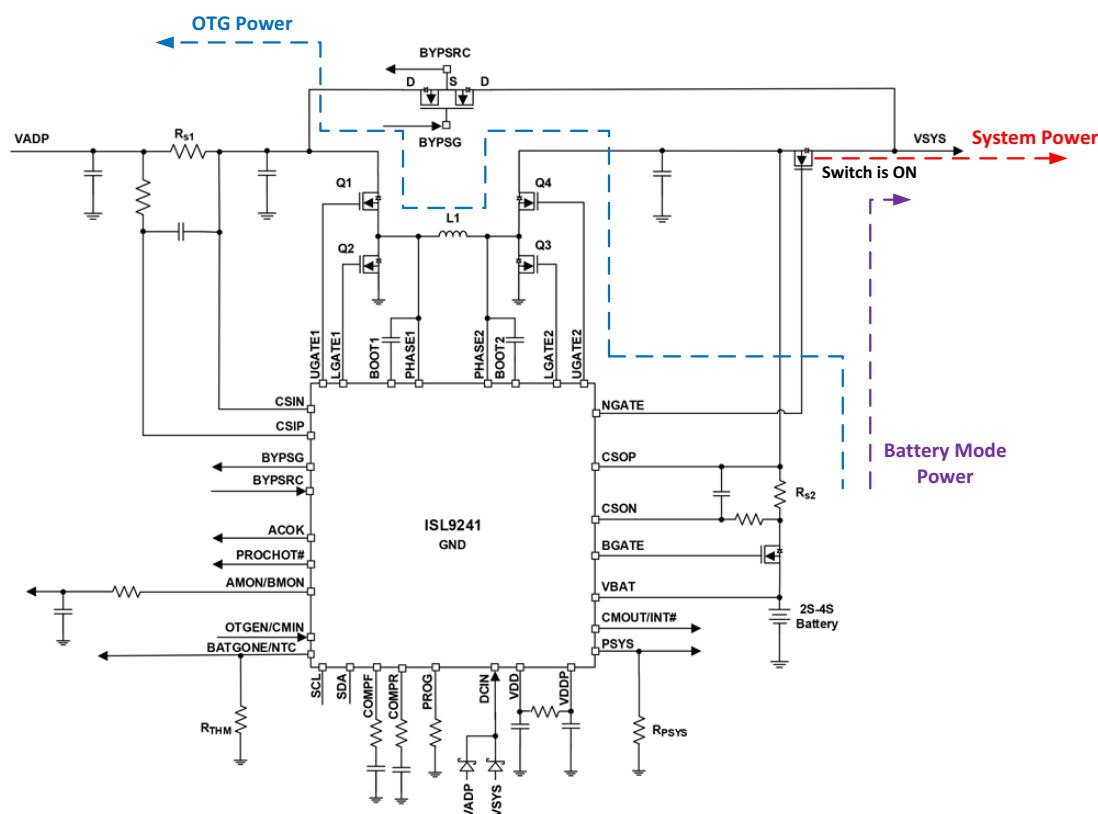
Figure 4. Battery Only Mode and OTG Mode
