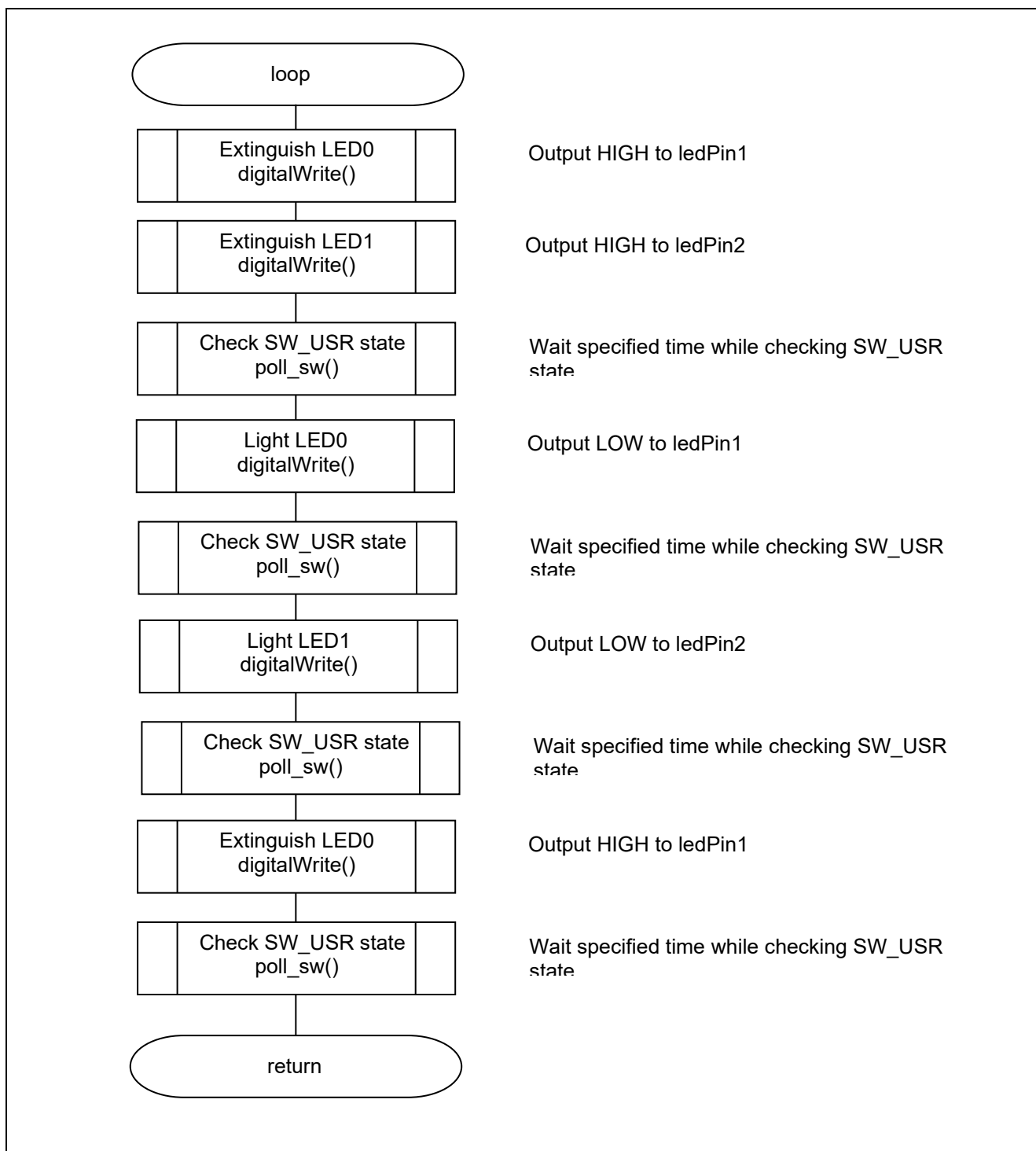
Figure 5.2 Main processing function
