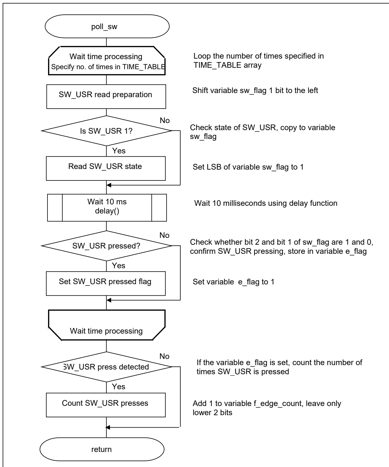
Figure 5.3 SW_USR check and wait time function
