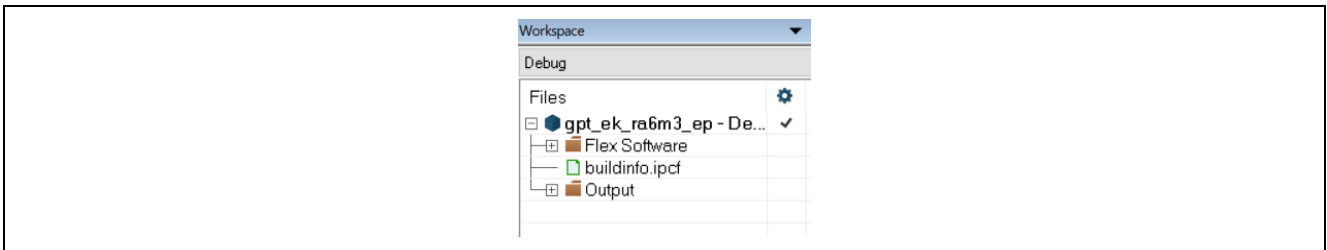
Figure 21. Project Structure
