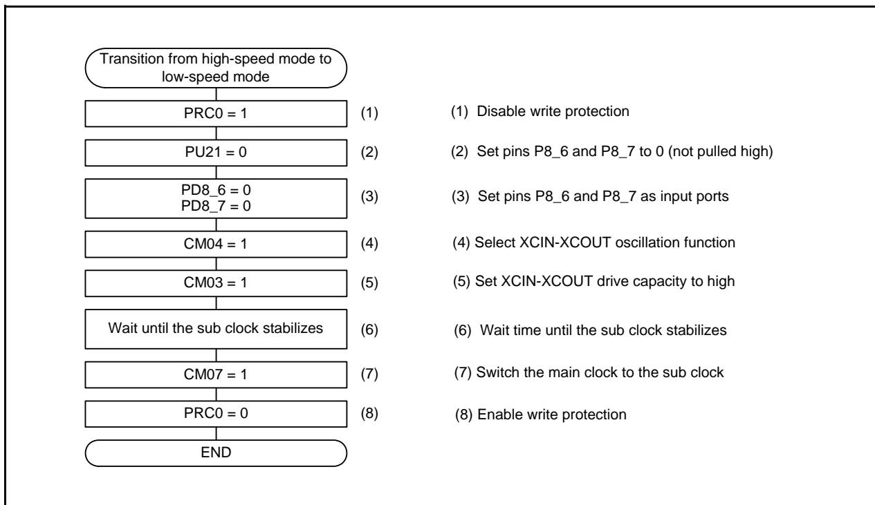
Figure 3.2 Transition Procedure from High-Speed Mode to Low-Speed Mode
