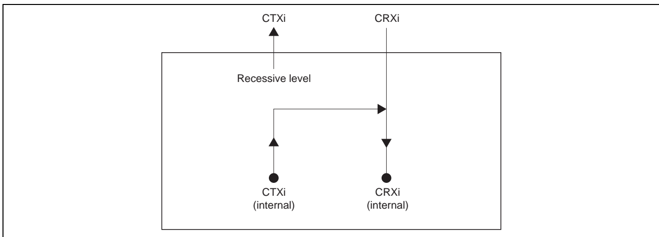
Figure 47 Listen-Only Mode Operation Illustration
