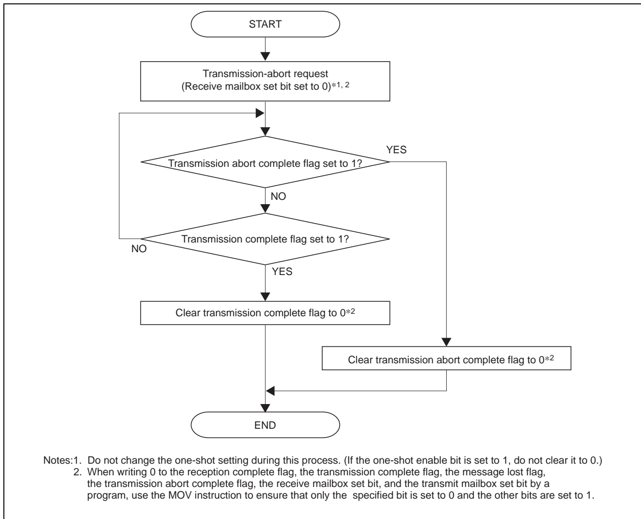
Figure 12 Transmission-Abort Procedure
