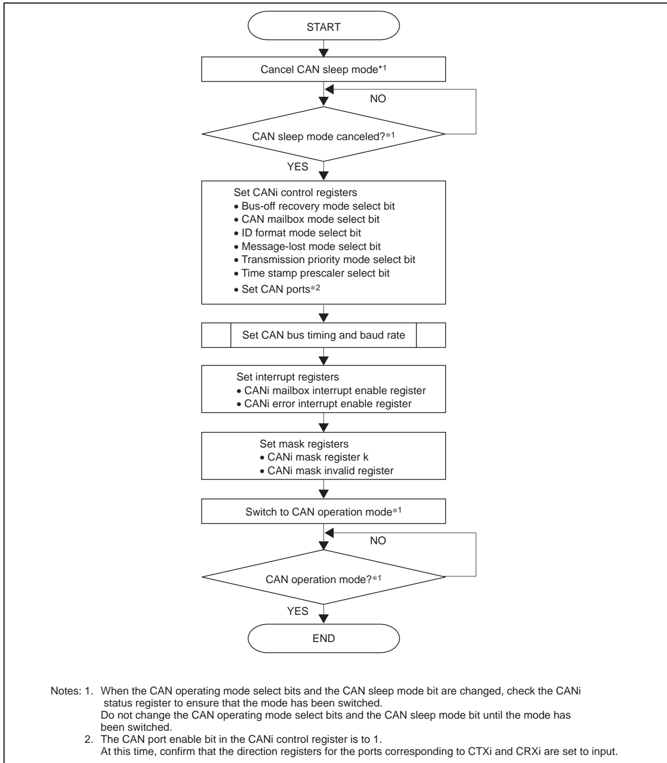
Figure 4 CAN Configuration Procedure after a Hardware Reset
