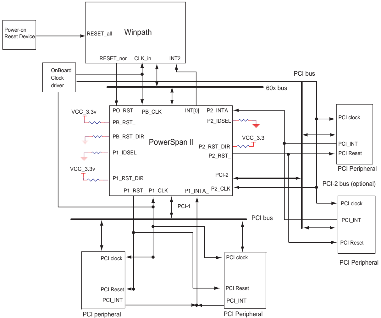
Figure 13: WinPath as the Host Processor
