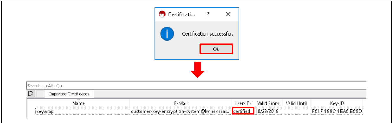
Figure 37. Successful Certification
