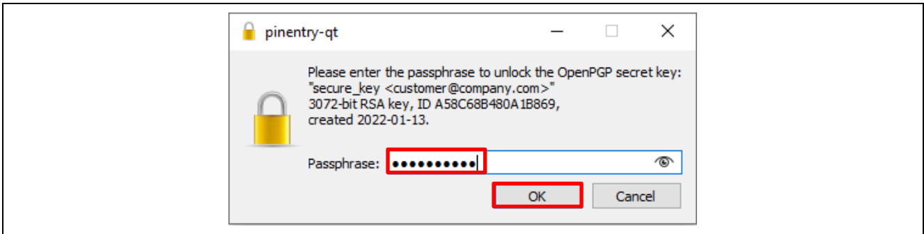
Figure 53. Provide Passphrase
