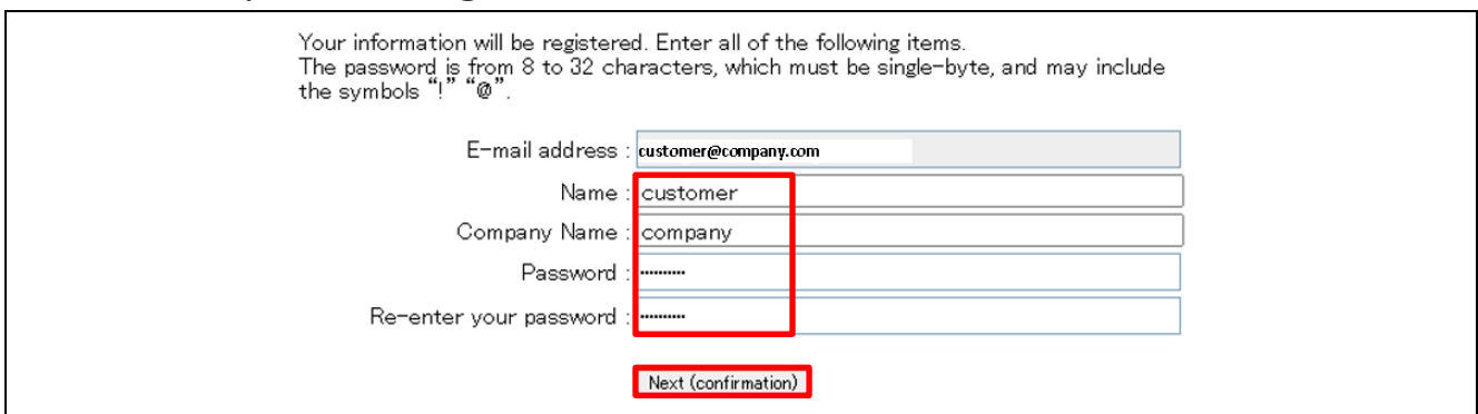
Figure 23. Confirm Registration
