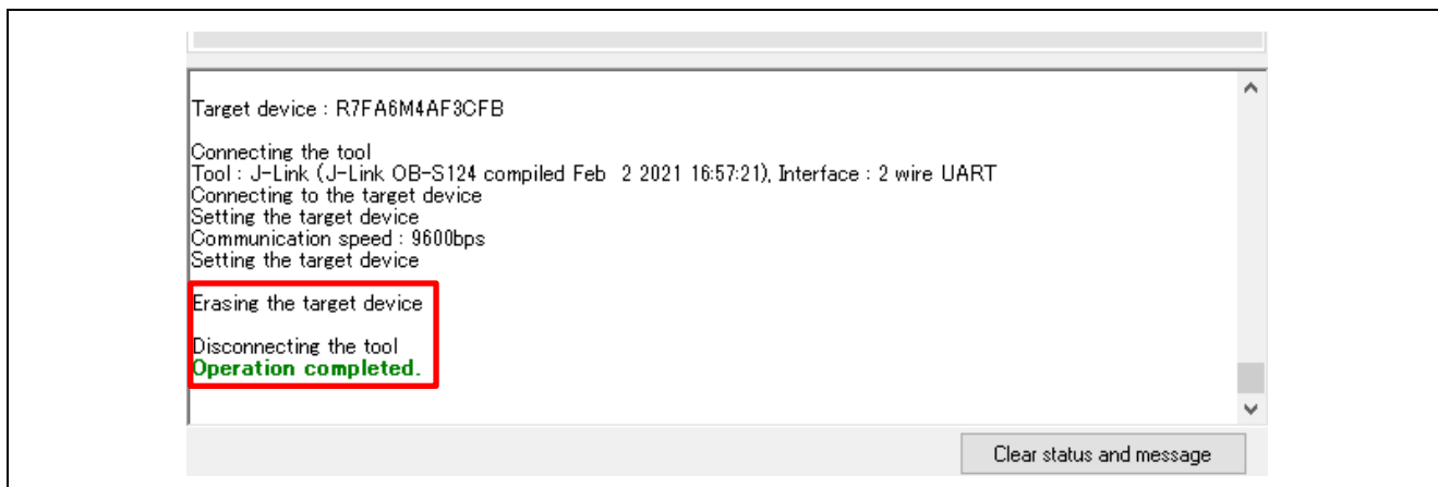
Figure 103. RA6M4 Initialization
