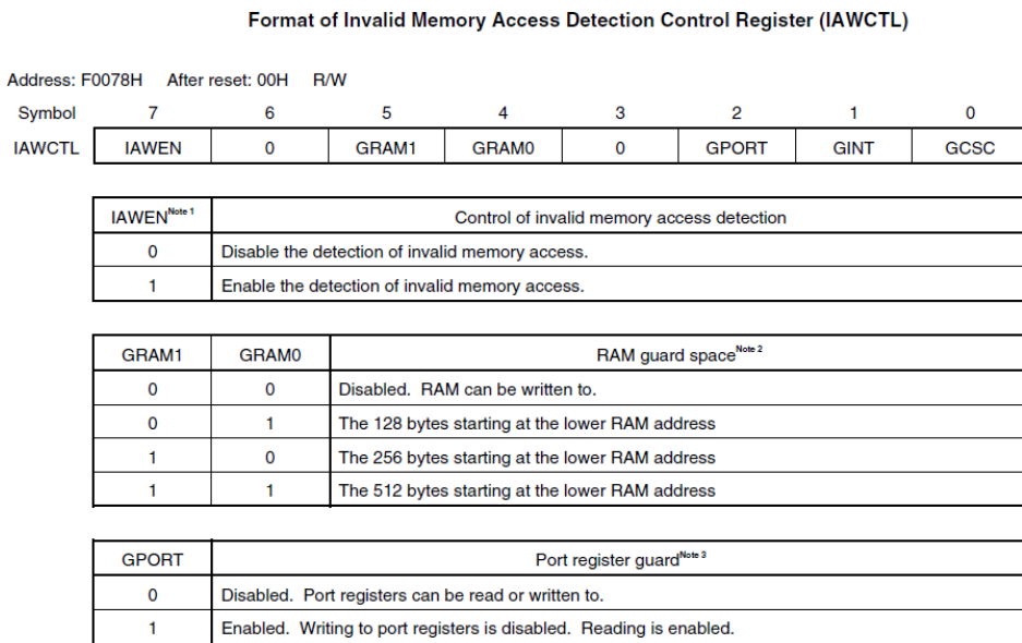
Figure 20: I/O Port SFR Guard Protection
