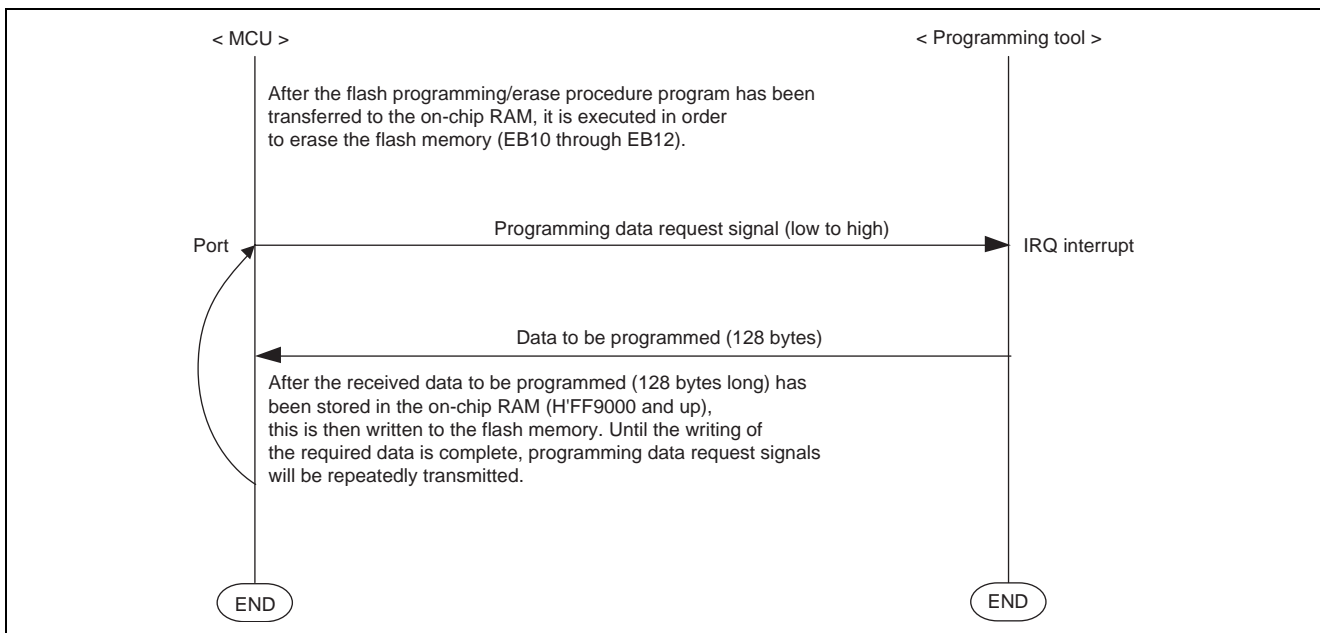
Figure 2 Control Operation
