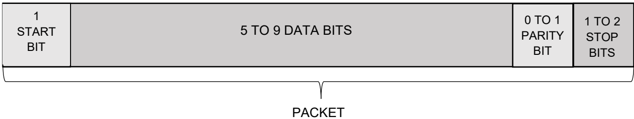
Figure 2: Data Frame for Receiver
