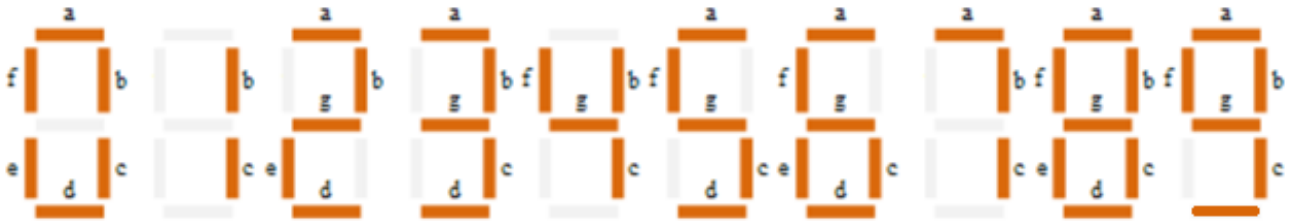
Figure 4: Digital Segments for all numbers
