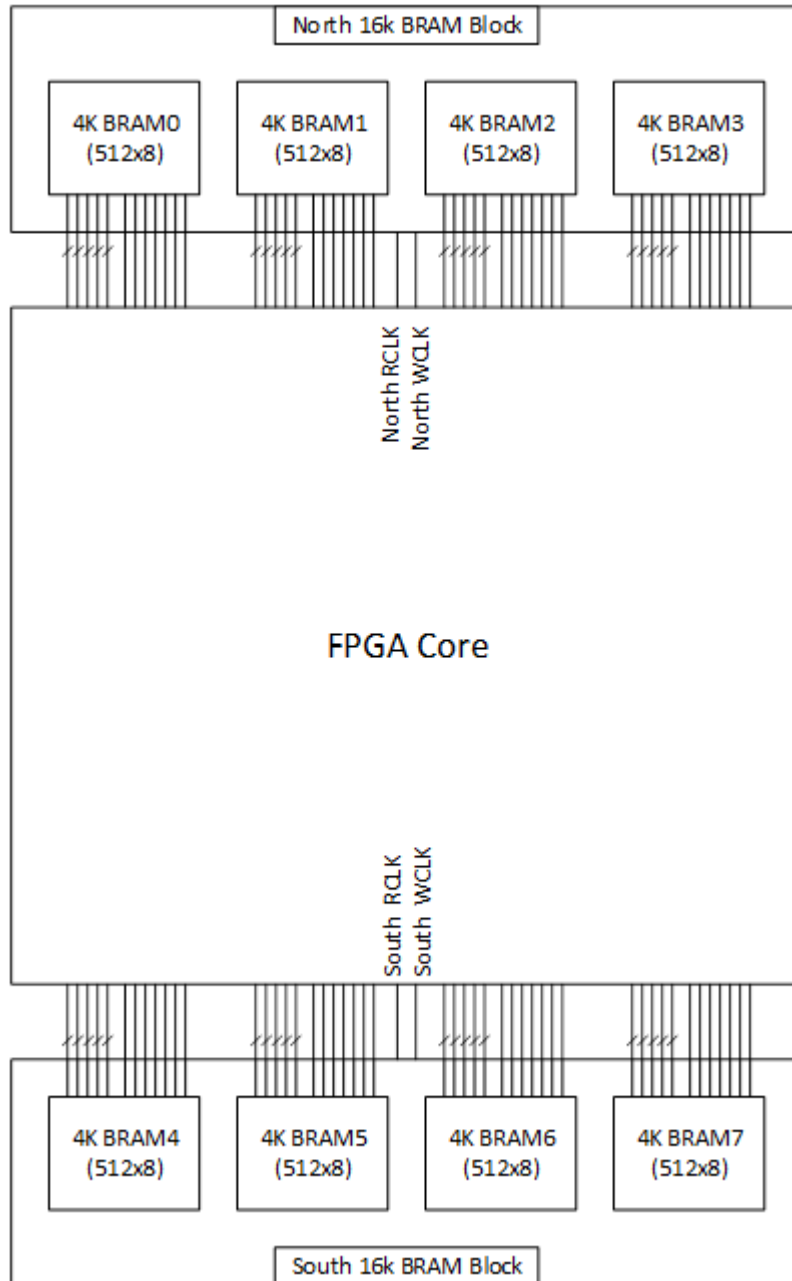
Figure 1: FPGA Core and BRAM Blocks
