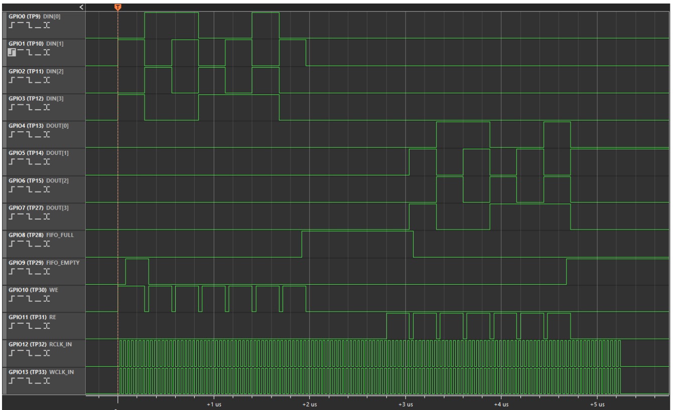
Figure 8: Output on Logic Analyzer
