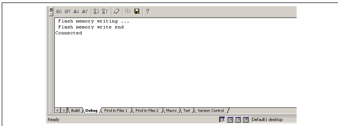
Figure 3.10 [Output] Window
