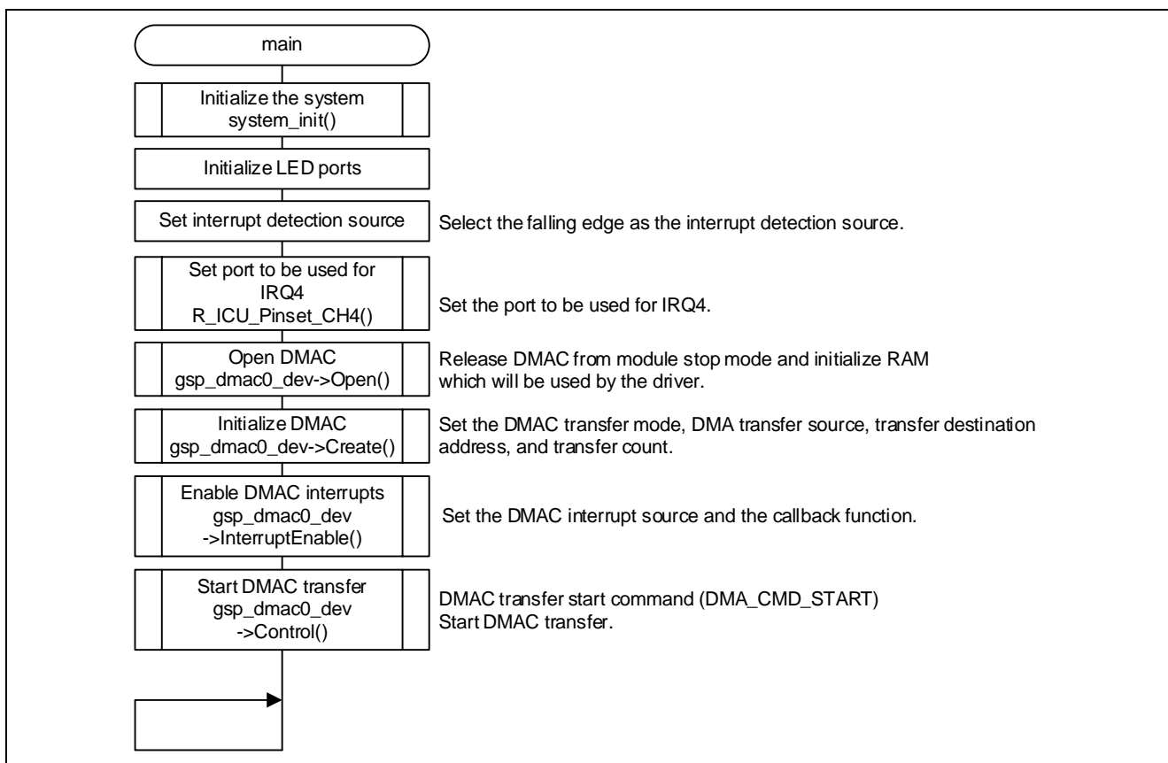
Figure 3.2 Main Processing
