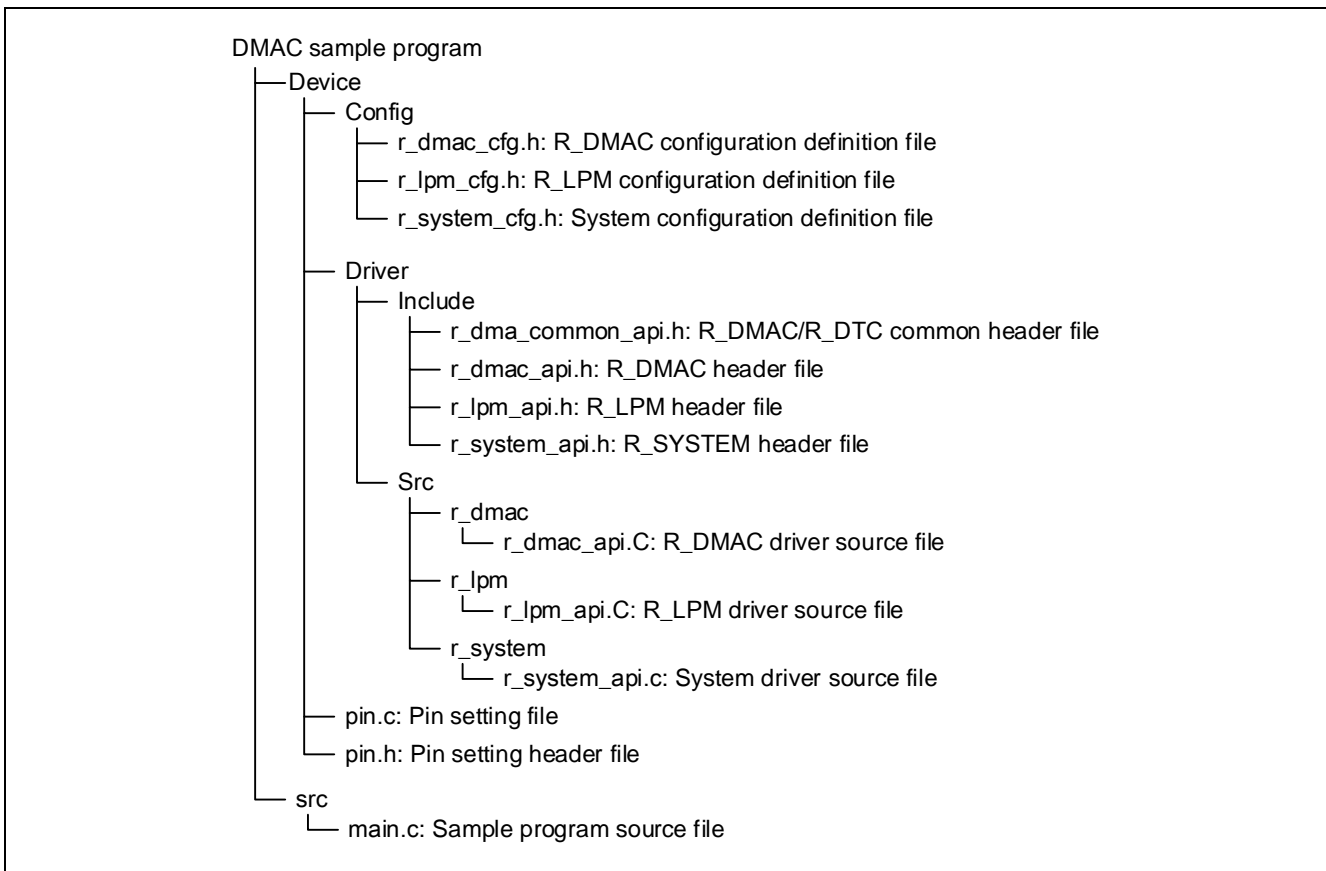
Figure 1.1 Folder Structure
