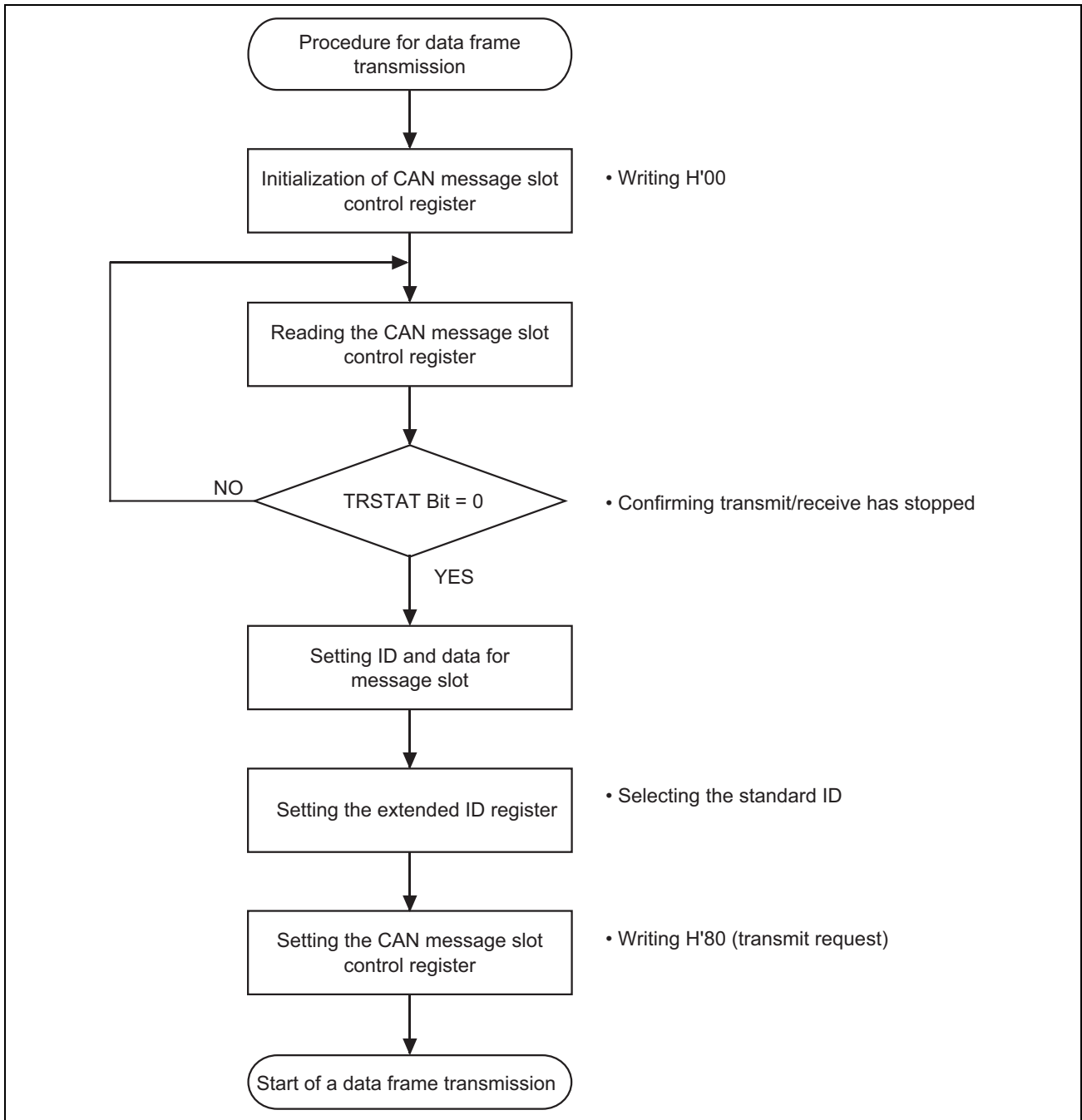
Figure 4.3.1 Data Frame Transmission Processing
