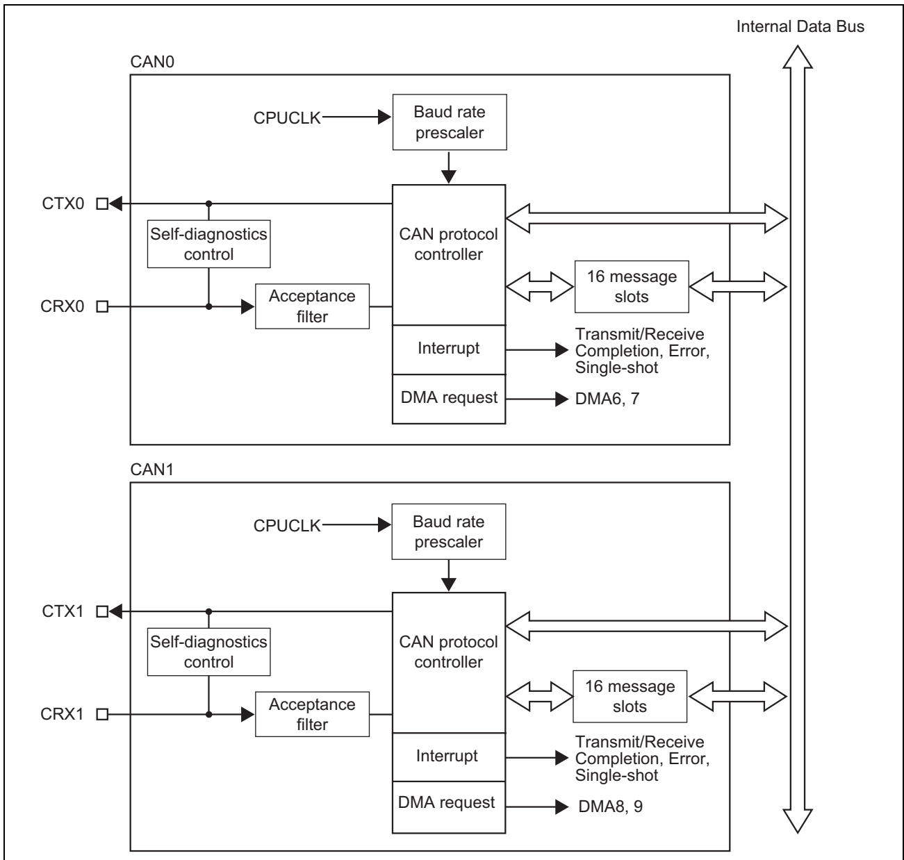
Figure 3.1.1 CAN Module Block Diagram
