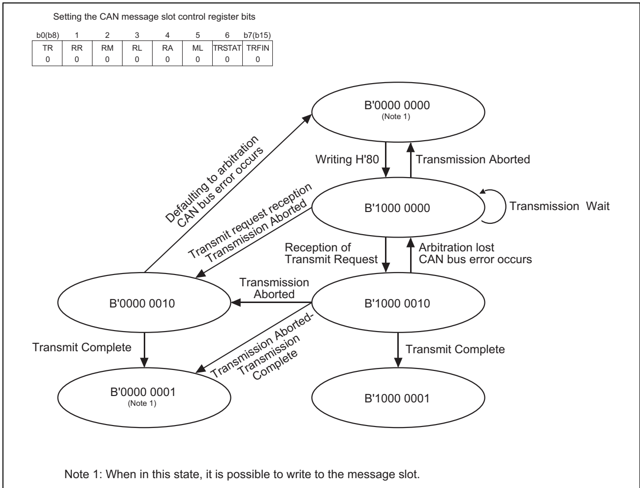
Figure 4.4.1 The State of CAN Message Slot Control Registers during Data Frame Transmission
