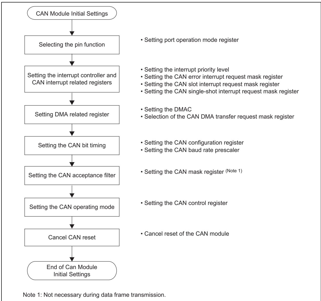
Figure 4.2.1 CAN Module Initial Setting
