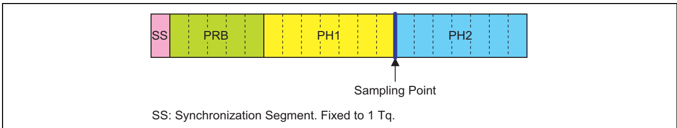
Figure 4.5.1 Bit Timing
