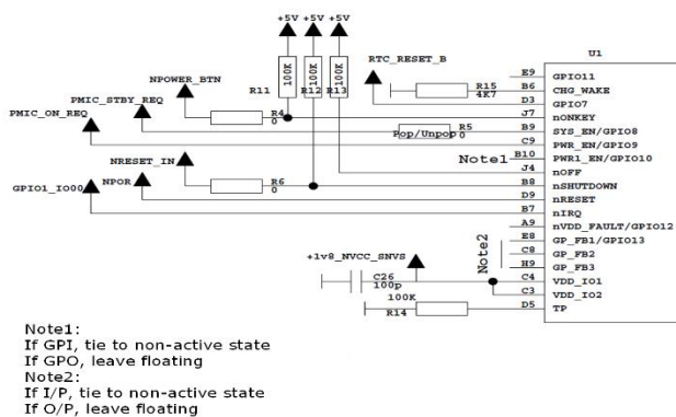
Figure 3: DA9063 i.MX8M Mini: Typical Application Schematics
