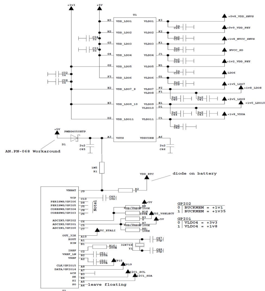
Figure 3: DA9063 i.MX8M Mini: Typical Application Schematics
