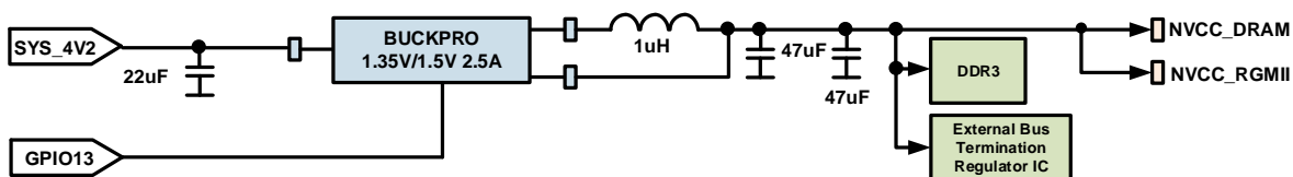
Figure 6: DDR3 Supply
