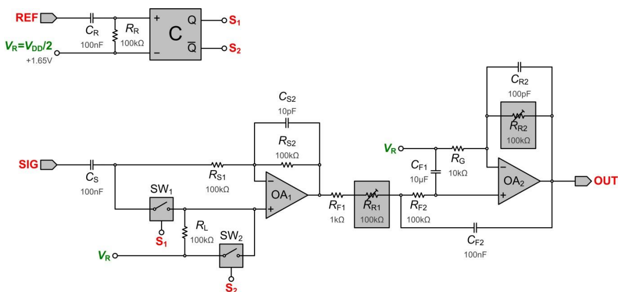
Figure 2: Principle of Operation of the Lock-in Amplifier
