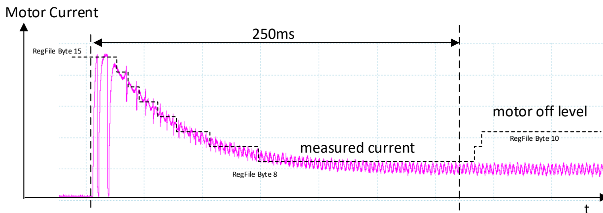
Figure 6: RegFile Usage
