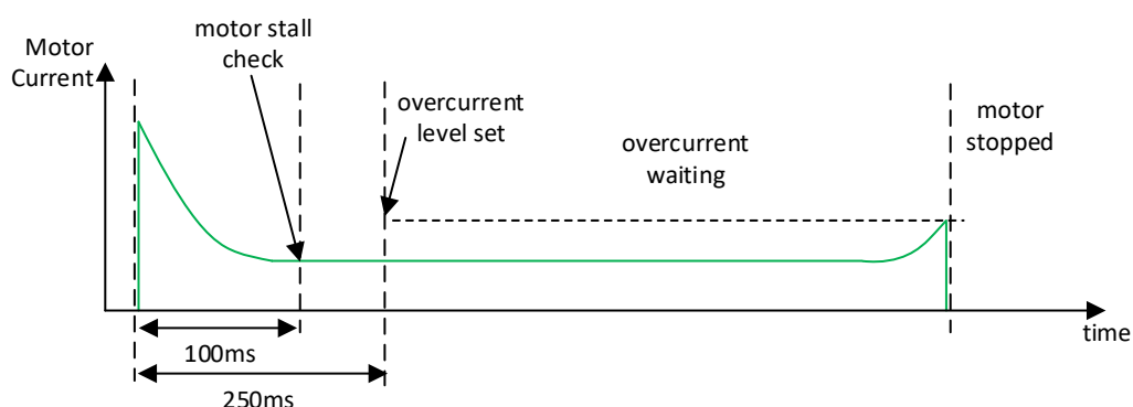
Figure 3: Design Operations
