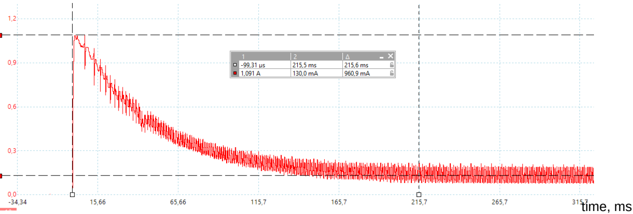
Figure 9: Motor Starting Current Waveform, Power Supply 3.6 V
