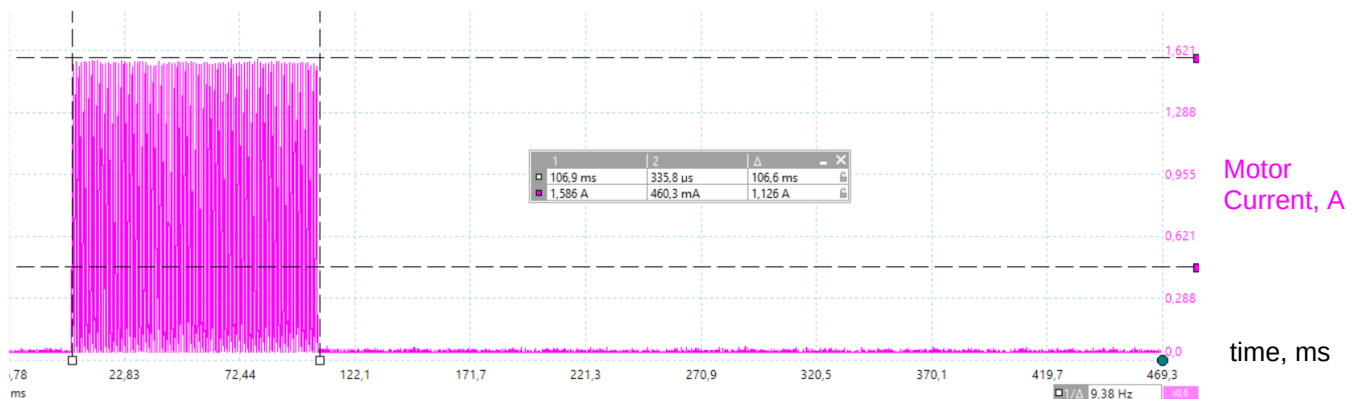
Figure 16: Stalled Motor, Power Supply 3.6 V – 6.0 V
