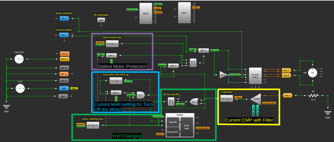
Figure 4: HVPAK Design
