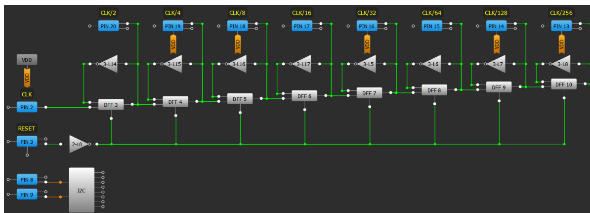
Figure 7: GreenPAK Design for the CD4024
