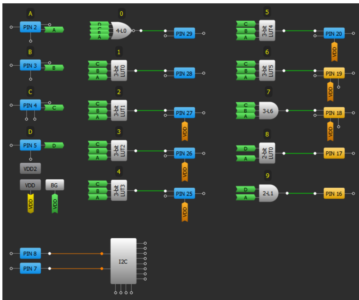
Figure 5: GreenPAK Design for the CD4028
