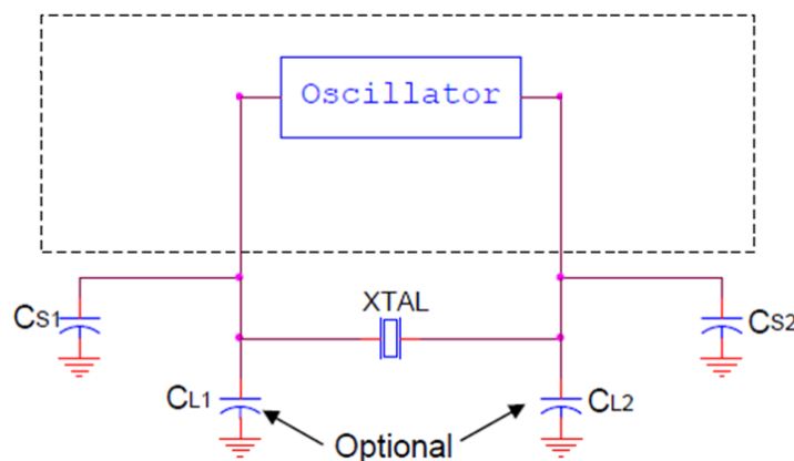
Figure 1. Crystal Capacitance
