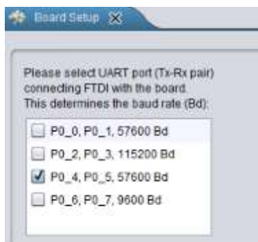
Figure 8: Board setup if UART is used
