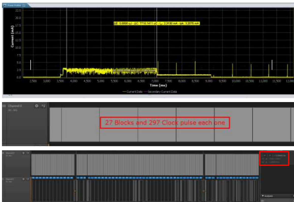
Figure 17: I2C memory mirroring into SRAM
