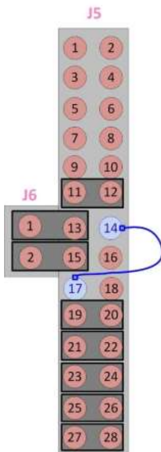
Figure 5: SPI Jumper Configuration with UART2 RX on Development kit-PRO
