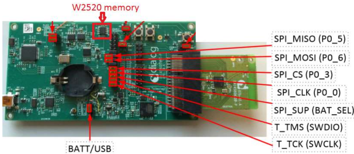
Figure 3: Development kit-PRO
