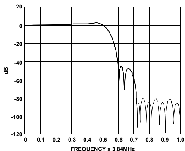
FIGURE 3. 38-TAP FIR FREQUENCY RESPONSE
