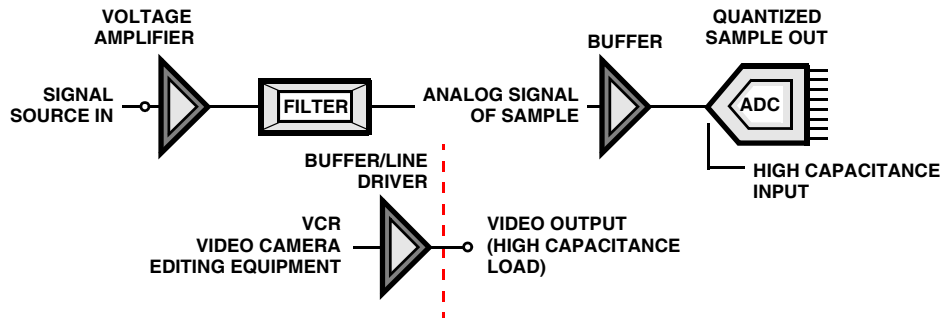
FIGURE 2. AMPLIFIER APPLICATIONS
