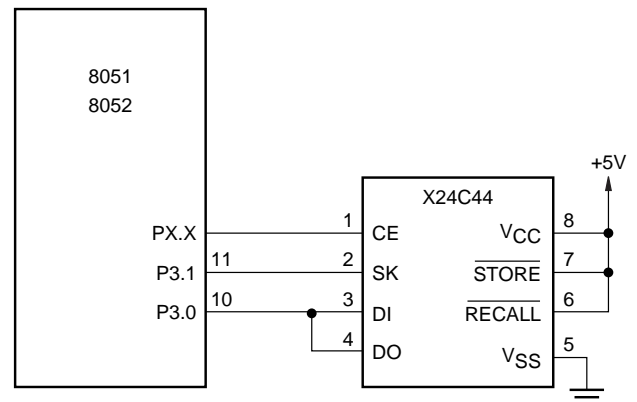
FIGURE 2. BASIC CONFIGURATION
