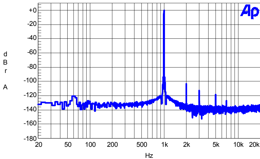
AUDIO PRECISION INTERSIL X9241A THD+N CHAN 0
