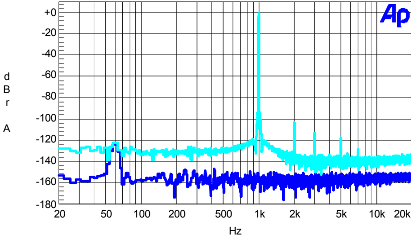
AUDIO PRECISION INTERSIL X9241A SNR CHANNEL 0
