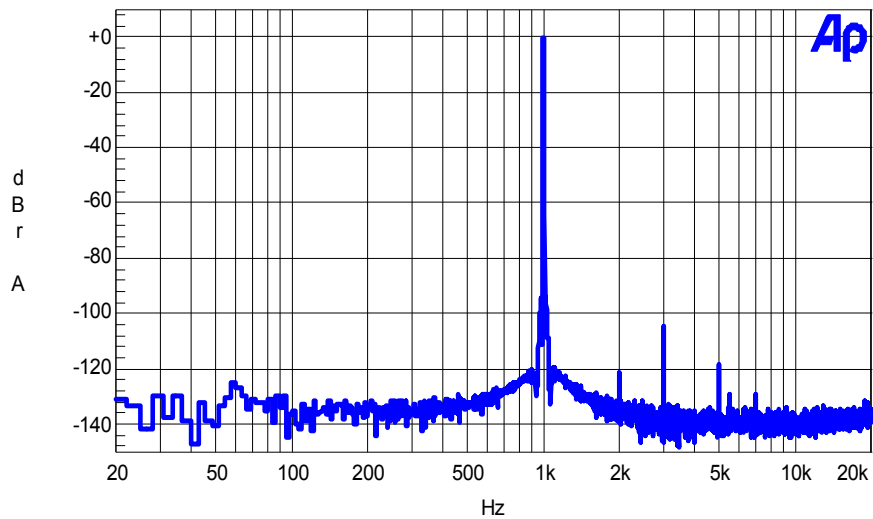
AUDIO PRECISION INTERSIL X9408 THD+N CHAN 0
