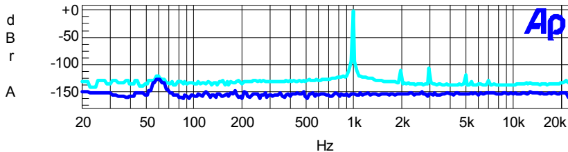
Audio Precision Intersil X9408 SNR CHAN 0
