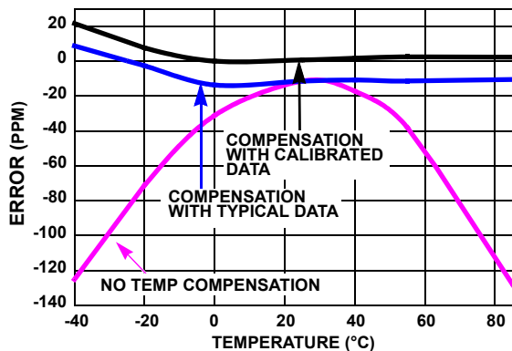
FIGURE 4. EPSON MC-156 ERROR vs TEMPERATURE (-40 °C TO +85 °C)
