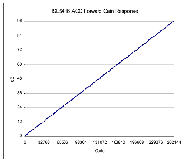
FIGURE 1A. AGC FORWARD GAIN
