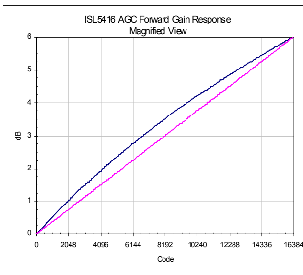
FIGURE 1B. MAGNIFIED VIEW
