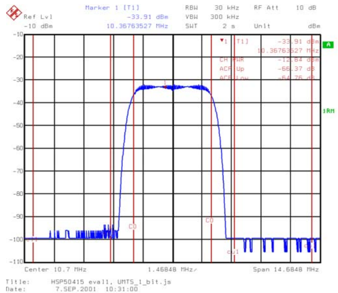
FIGURE 3. ANALOG SPECTRUM
