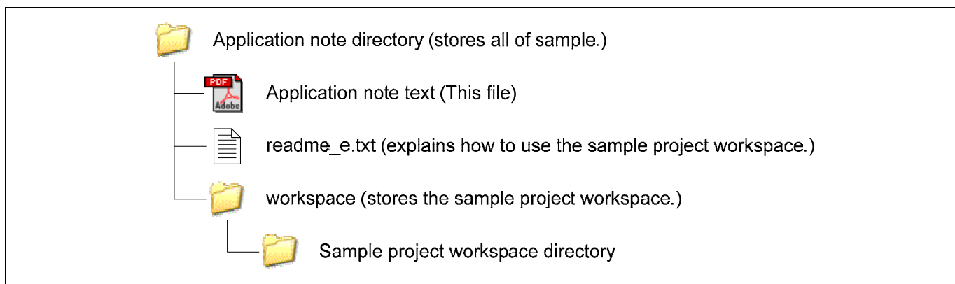
Figure 1.1 Directory Configuration
