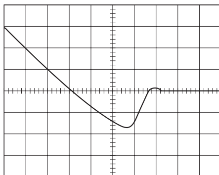
2SK1671 ( i_F = 30A, d_i/d_t = 100A/\mu s )
