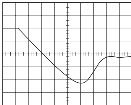
2SK1170 ( i_F = 20A, d_i/d_t = 100A/\mu s )
