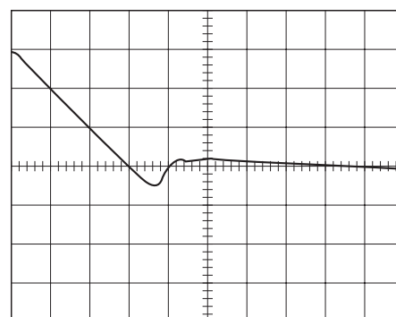
2SK1669 ( i_F = 30A, d_i/d_t = 100A/\mu s )
