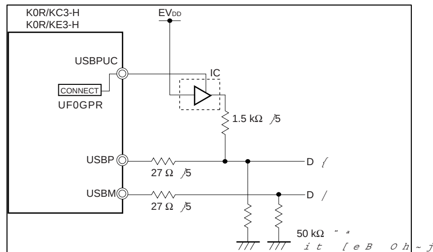
Figure 3-4 USB function controller Connection Example
