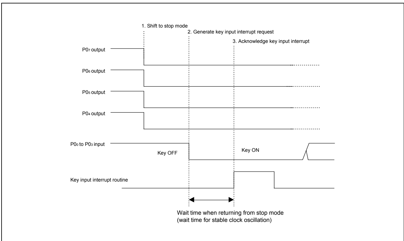
Figure 3.2 Example of Key Input Interrupt Operation Timing in Stop Mode
