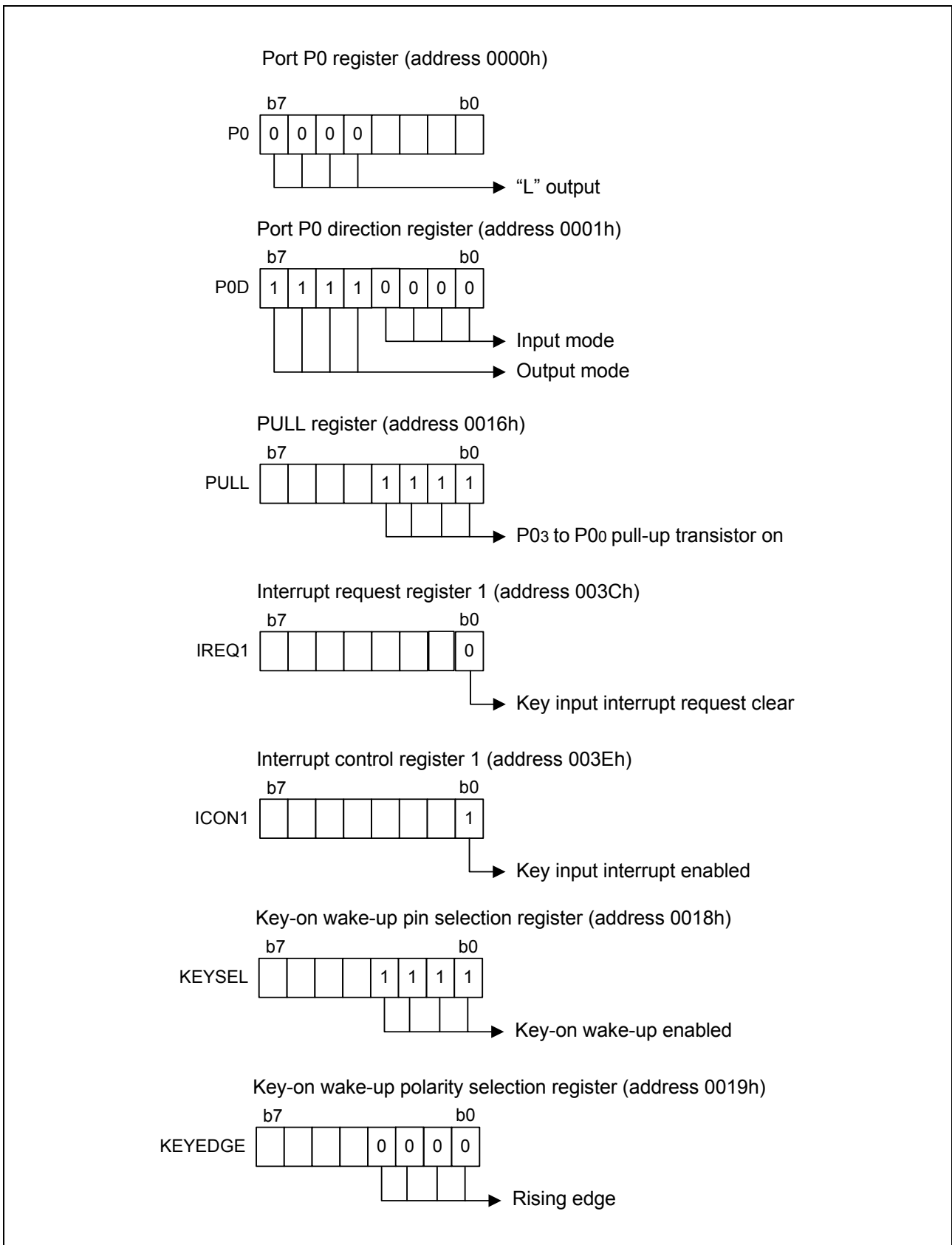
Figure 3.3 Relevant Register Settings
