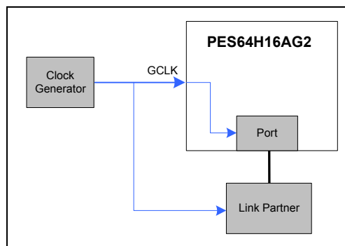
Figure 2 Global, Common Clocked Configuration
