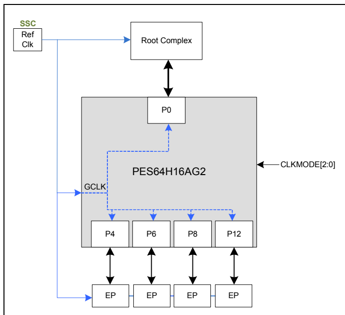
Figure 6 Typical Server/Desktop System Clock Usage Model
