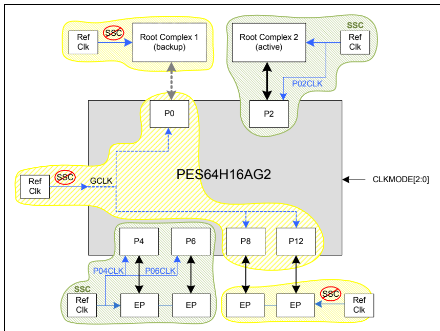
Figure 9 System Clock Configuration #3
