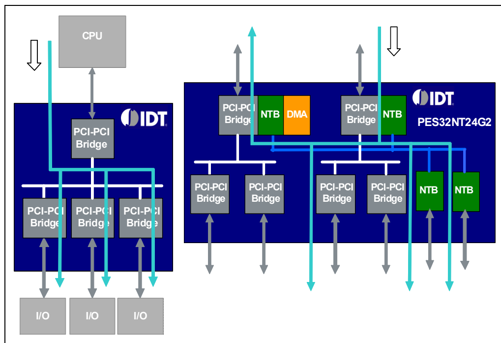
Figure 9 Possible Multicast Data Path
