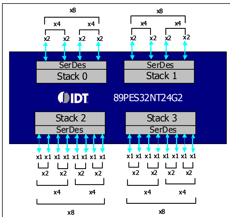
Figure 1 Block Diagram
