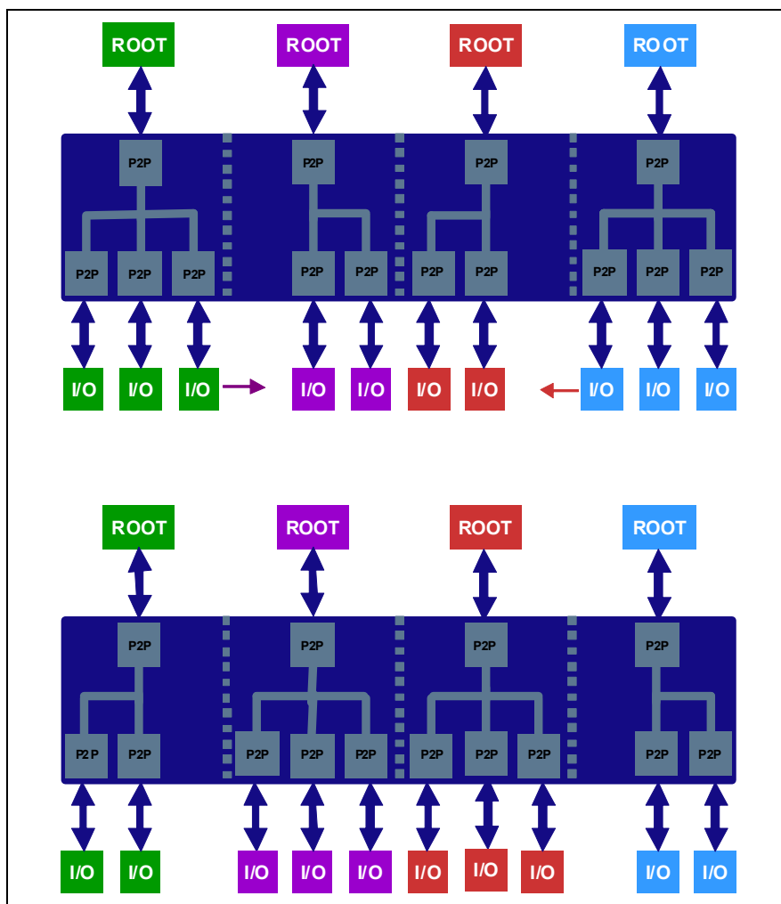
Figure 4 Dynamic Redistribution of I/Os
