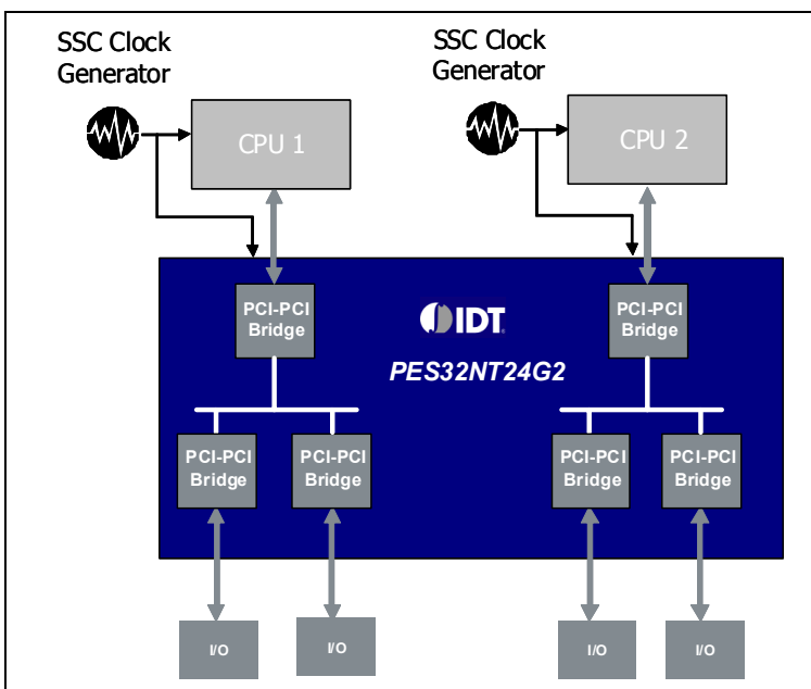
Figure 13 Multiple SSC Clock Domains
