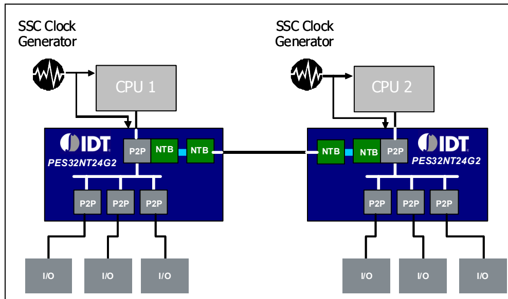
Figure 14 Multiple SSC Clock Domains Across Multiple Switches
