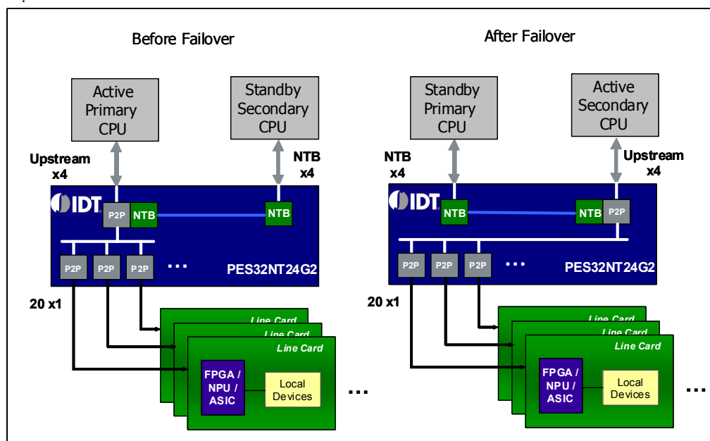
Figure 10 Dual-Host Failover System
