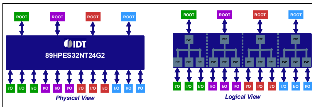
Figure 3 Switch Partitioning
