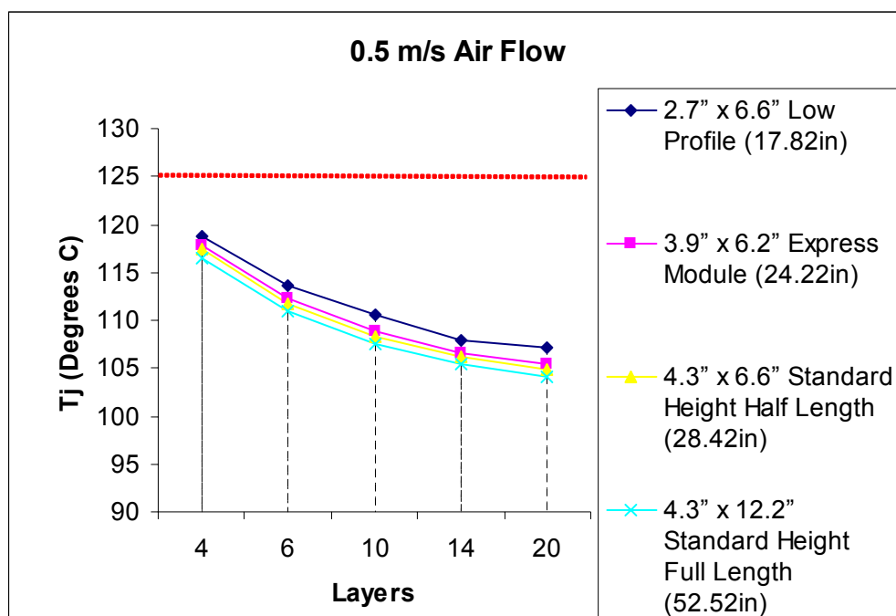
Figure 8 PES24T6G2 Heat Sink Requirements with Air Flow
