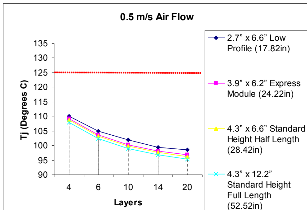
Figure 6 PES24T3G2 Heat Sink Requirements with Air Flow
