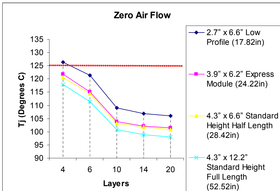
Figure 1 PES16T4AG2 Heat Sink Requirements without Air Flow
