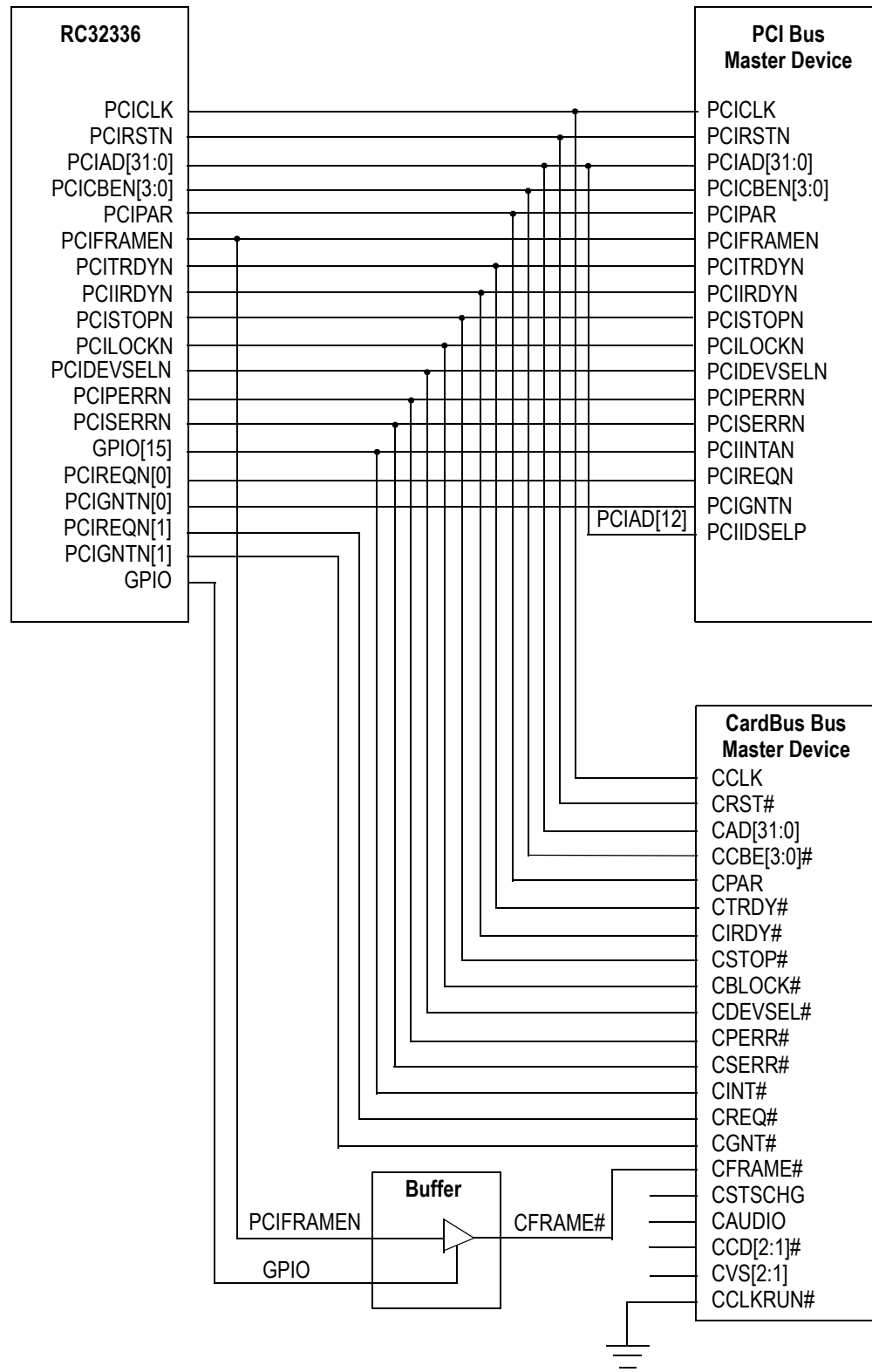
Figure 3 Connection Between the RC32336, a PCI Bus Master Device, and a CardBus Bus Master Device
