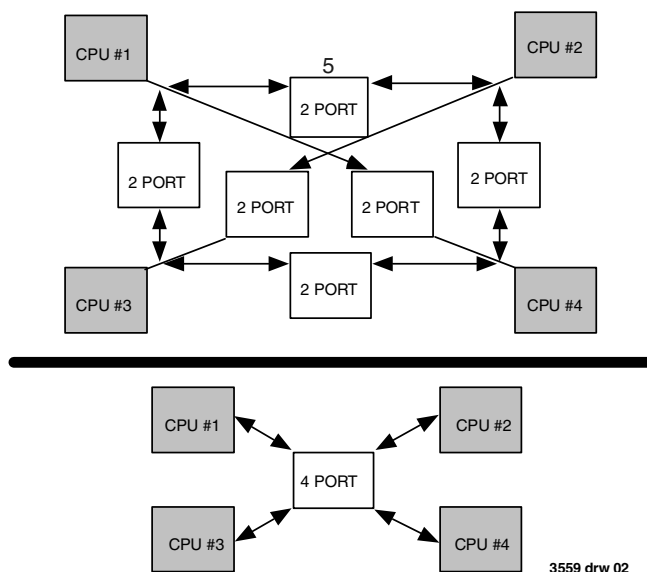
Figure 2. FourPort™ SRAM interconnection advantages over Dual-Port SRAM. The processors in both figures are interconnected with a latency of one memory access. This efficiency requires 6 separate Dual-Port SRAMs but only 1 FourPort™ SRAM.
