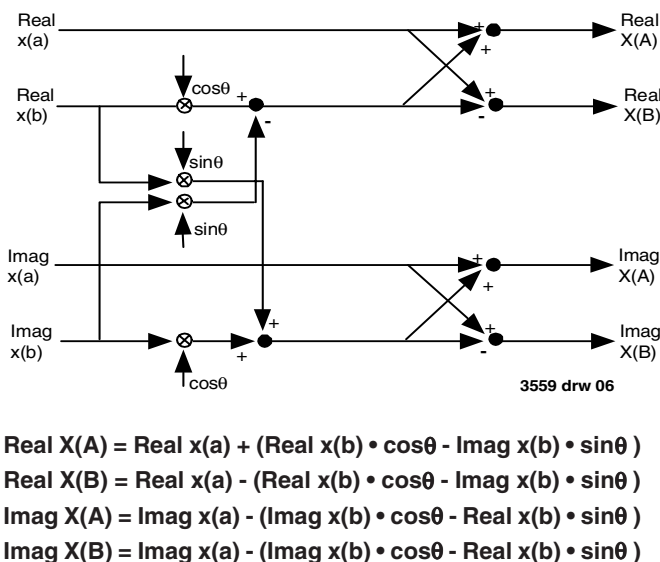
Figure 6. Flow Diagram for Calculating One FFT Butterfly. Each "X" pattern shown in Figure 5 represents one such "Butterfly". Each end point in Figure 5 represents a complex pair of numbers input or output to or from a "Butterfly". The sine and cosine factors are sometimes called "Twiddle Factors". The angles used for calculating the Twiddle Factors for each Butterfly are shown in Figure 5.
