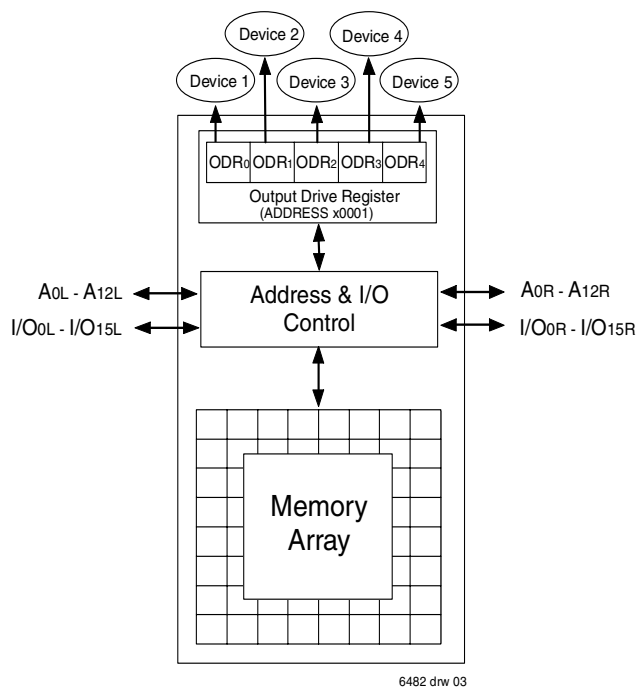
Figure 3. IDT70P248 Output Drive Register
